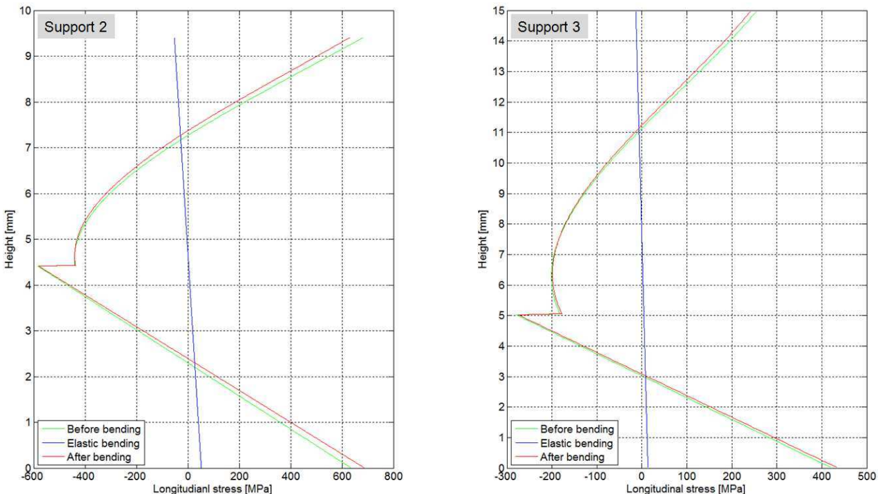
Fig. 5 Eigen stresses before and after bending effects
