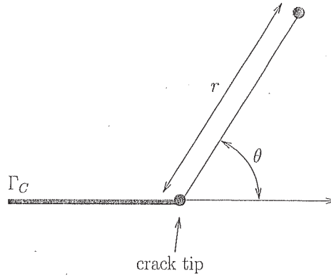
Figure 2. Polar co-ordinates relatively to the crack tip.
