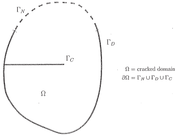
Figure 1. A cracked domain.
