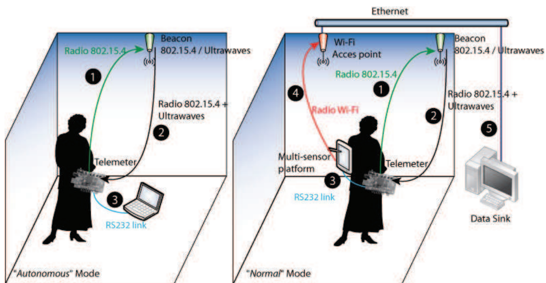
Fig. 1. System architecture with two possible modes.
