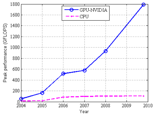
Fig. 1. CPU versus GPU evolution
