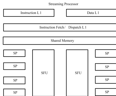
Fig. 2. GPU Architecture
