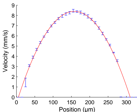
Fig. 5 A comparison between theoretical profile (solid red curve) and 8 consecutive measured profiles (blue errorbars) along the centre-line of the flow channel with a flow speed of 20 \mu\text{L}/\text{min}^{-1} . The liquid is milk (2 %) diluted in water
