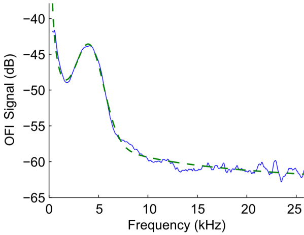
Fig. 3 OFI signal in frequency domain measured at the middle of the channel and the corresponding fitting curve (Eq. (6)). The mean frequency in the sensing volume is calculated by extracting the Doppler frequency of the signal
