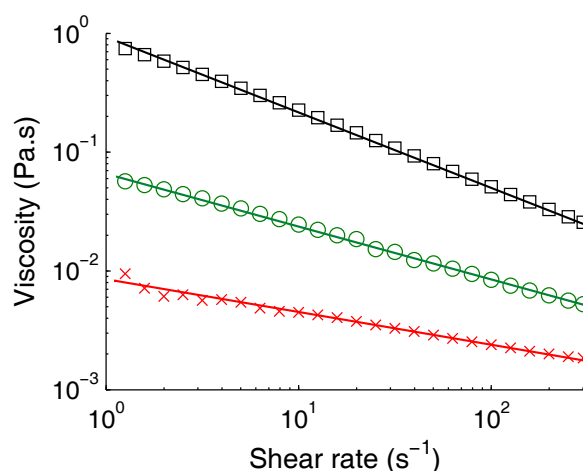
Fig. 7 Experimental rheograms for various concentrations of xanthan gum (0.25 (cross) 1 (circle) and 3 g/L (square)). The viscosity of each solution as a function of the shear rate applied are plotted in logarithm
