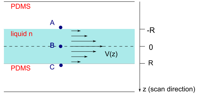
Fig. 2 Diagram showing the scan configuration with respect to the z -axis of the flow channel. The angle calibration is calculated at position B, and the velocity profile is measured from A to C. The flow channel has a 160 \mu\text{m} internal radius R
