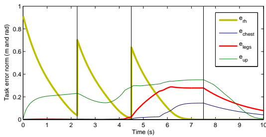
Fig. 30: Experiment C: Norm of the task errors.
