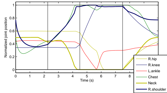
Fig. 32: Experiment C: Normalized joint positions.
