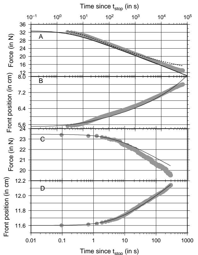
FIG. 7: Variation of force, F and front position \bar{a} obtained during the relaxation regime for the experiment displayed on Figure 2 and for 5 minutes (gray dots, C and D). Results of the numerical integration are represented as black line. Same representation is made for the experiments monitored for more than 18 hours in the relaxation regime and is displayed in the two upper graphs (A and B). The dashed line shows the evolution of force deduced from the fit of the front position from Eq. 1.
