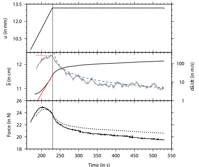
FIG. 2: Top : Variation of loading point position, u , as a function of time during an experiment. At time t = 230 s , the loading point is maintained in a fixed position. Middle: Variation of the average front position, \bar{a} , as a function of time (black solid line) and evolution of the crack front velocity d\bar{a}/dt (gray solid line). The red solid and dashed lines represent a fit to the average front position and velocity, respectively, according to Eq. (18). The blue dashed line is a fit to the crack velocity in the relaxation regime following Eq. (25). Bottom : Variation of force as a function of time (black solid line) and force predicted by the beam theory (dark dashed line) using (5) with E = 3.2 GPa , h = 4.9 mm and b = 2.84 cm which are the measured properties of the plate. For all figures, the vertical gray line denotes the time at which the loading was stopped and separates the imposed velocity regime from the relaxation regime.
