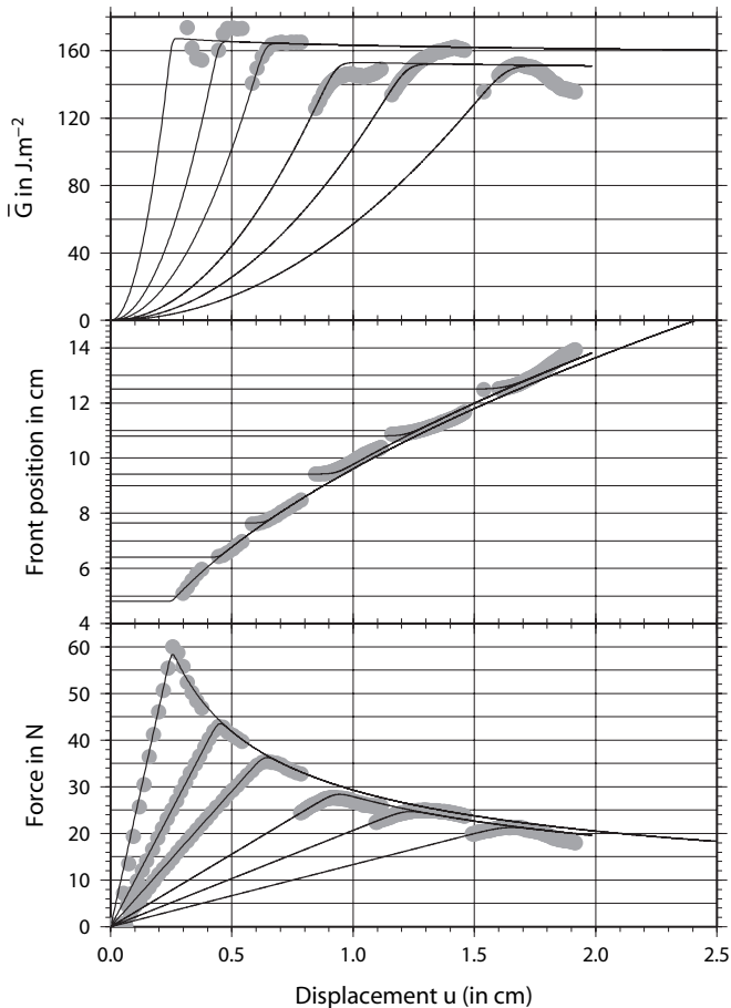
FIG. 6: Variation of force, F , front position \bar{a} and energy release rate, \bar{G} , obtained during six experiments (gray points) carried in the forced regime. The results of the numerical integration of Eq. (13) are drawn as black lines. The model captures most of the features observed in our experiments, such as the peak value of the force and its occurrence time. It also captures the appearance of a Griffith regime, i.e. the fact that \bar{G} is close to constant at large enough crack speed.
