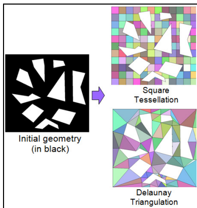
Figure 5. Example of Tessellations (square and triangle).
