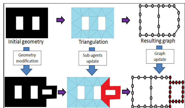
Figure 13. Example of a local modification of a graph
