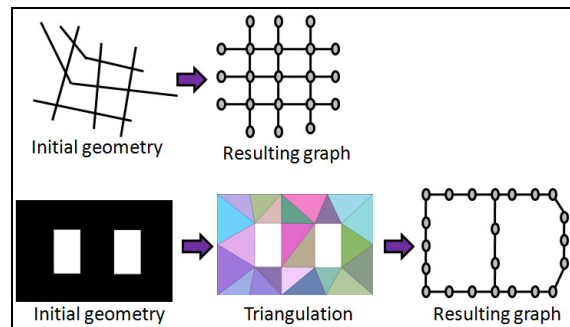
Figure 7. Example of graph computation
