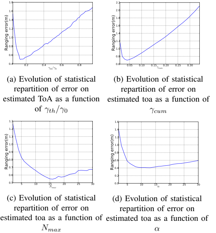
Fig. 9. Tuning of different ranging techniques using UWB measurements: the key-parameters are chosen to best fitting the measurements.
