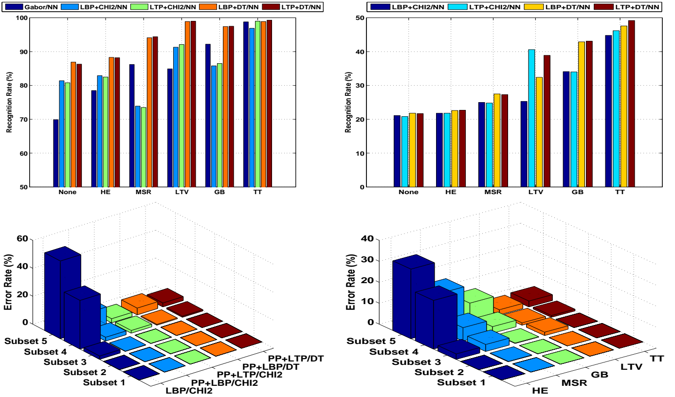
Fig. 12. (Top) Overall nearest-neighbor recognition rates (%) on (left) Extended Yale-B and (right) CAS-PEAL-R1, using the proposed LBP based and Gabor features and various preprocessing methods. (Bottom) Breakdown of error rates on the five Extended Yale-B subsets for (left) the various feature sets with our standard preprocessing, and (right) the various preprocessing methods with LTP/DT features.
