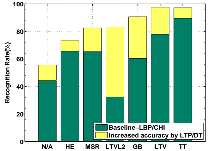
Fig. 18. Improvements due to replacing LBP/ \chi^2 with the less noise-sensitive features LTP and the more robust similarity metric DT, for various illumination preprocessors on Extended Yale B set 5.
