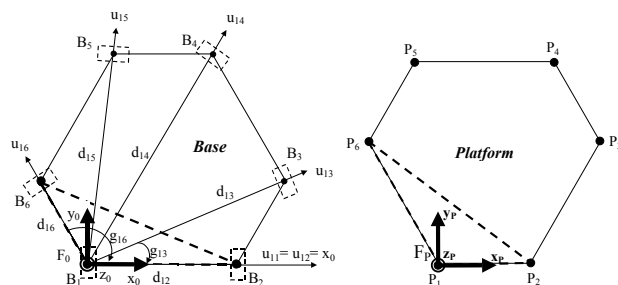
Fig. 2. Frame F_0 fixed with the base and frame F_p fixed with the mobile platform.
