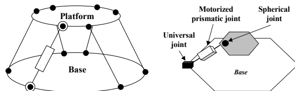
Fig. 1. Description of the 6 degree of freedom Gough-Stewart robot.
