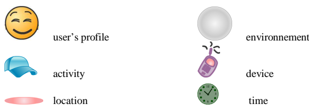
Figure 3. Avatar
