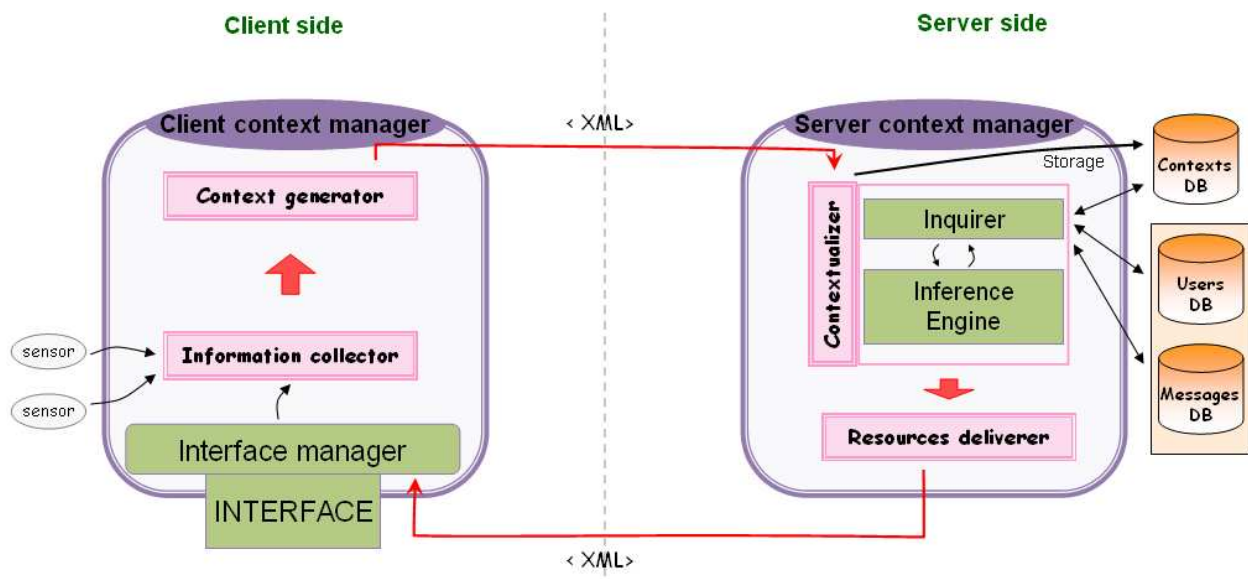
Figure 2. MeCoCo architecture
