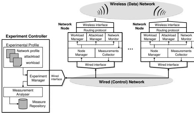
Figure 1. Experimental platform architecture.
