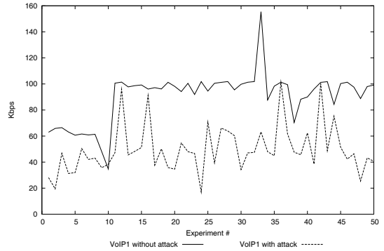
Figure 4. Impact of grey hole attacks on the goodput of experiments in a given campaign.
