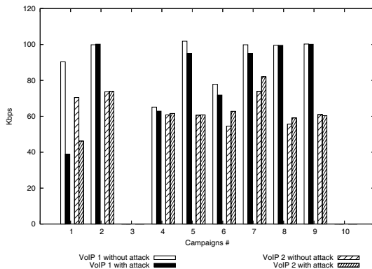
Figure 3. Impact of grey hole attacks on the data flow goodput of considered campaigns.
