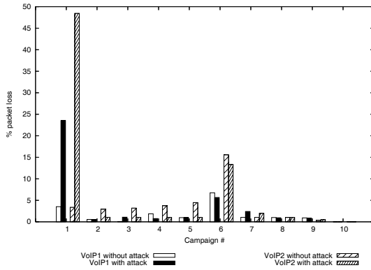
Figure 6. Impact of grey hole attacks on the packet loss rate of considered campaigns.
