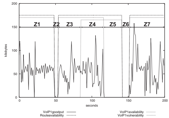
Figure 8. Data flow goodput versus route and data flow availability and vulnerability.
