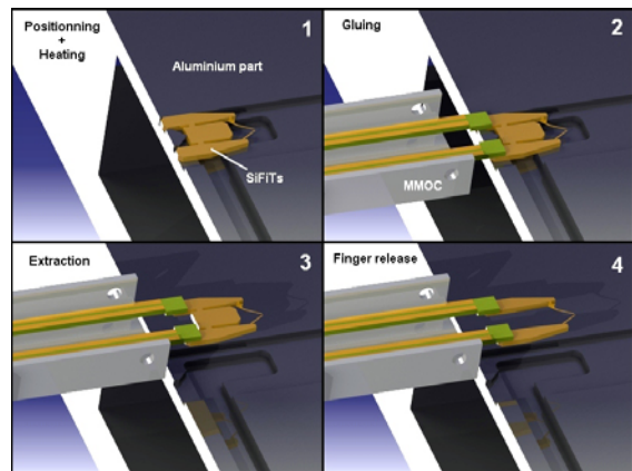
Fig. 6. Microgripper mounting process
