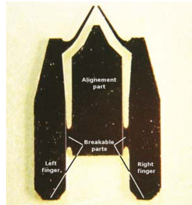
Fig. 5. Silicon Finger Tips - Before microgripper mounting process
