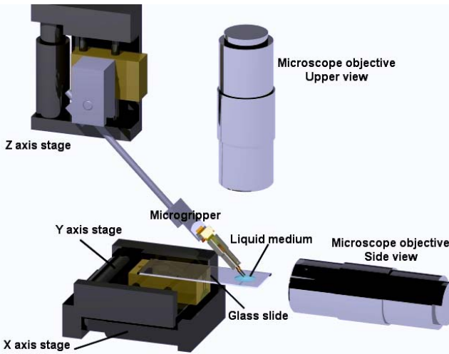
Fig. 2. Station setup
