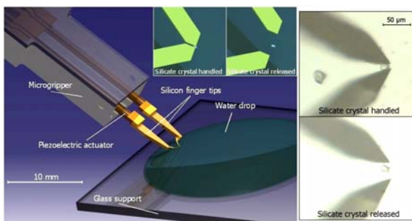
Fig. 8. Silicate crystal micromanipulation (virtual and real)
