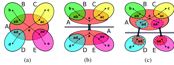
Figure 6: Another example of disconnected classes. (a) the original diagram, built without particular constraints. Let us now assume class D and E are not reachable from A, B, C . (b) the diagram obtained when representing the zone a as two separated regions. In this case, node duplication is generally not meaningful for a better comprehension of the diagram. (c) the same graph obtained duplicating the zones ad and ae and their nodes. Again, node duplication can be made clear by using a dashed line for the boundary. Although this solution allows us to see all the nodes of the same class in a connected region, it tends to be less readable than the previous one because of the greater number of extra links required.
