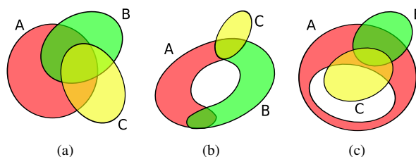
Figure 1: Euler diagrams as studied by different authors. (a) shows Euler diagrams as studied in [5]. They do not permit overlapping lines and multiple-line crossing points. (b) shows the more general Euler diagrams studied in [3]. Multiple line crossing point and overlapping boundary are allowed, as well as disconnected overlaps between the same sets. (c) shows Extended Euler diagrams (EED) as defined in [9]. Holes inside the sets are permitted.
