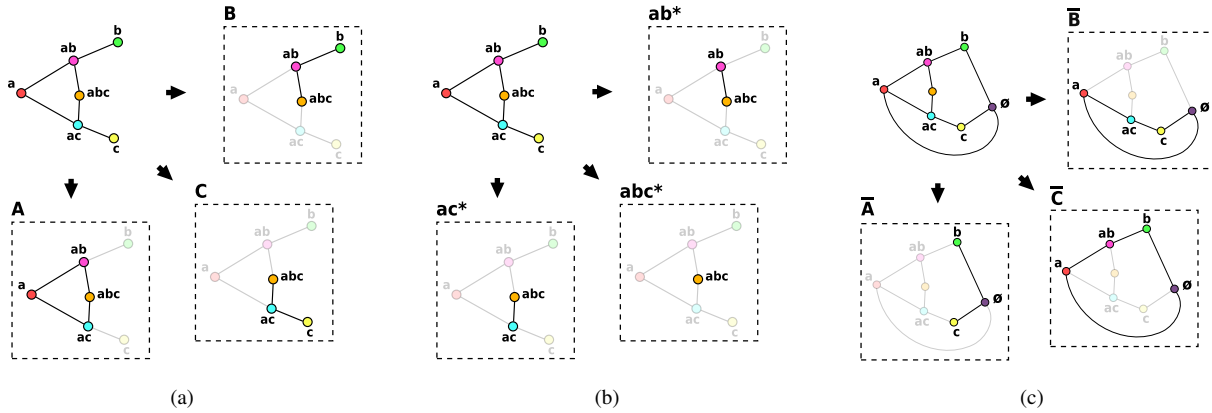
Figure 7: Some tests on the intersection graph. (a) checking that all the class schemas are connected. (b) checking that subgraphs induced by the nodes containing any possible subset of classes are connected. Here the subgraphs induced by the nodes containing ab , ac , and abc are shown. Together with the ones containing a , b , and c (that correspond exactly to the class schemas in the previous picture), they are all the possible non empty subgraphs of this kind. (c) checking that the complementar class schemas are connected. At this point we need to consider also a node associated to the external area, that will always be part of the complementar class schemas.
