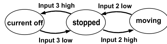
Fig. 3. Motor controller finite state machine
