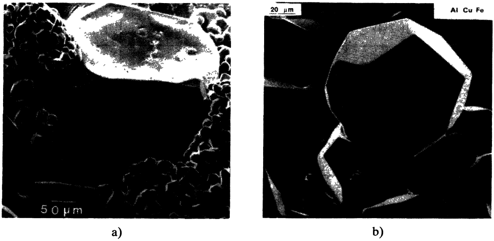
Fig. 7. — (a) Scanning electron micrograph of the single-phase \text{Al}_{63}\text{Cu}_{25}\text{Fe}_{12} alloy initially rapidly quenched and then annealed for 4 days at 1 143 K, showing a large single quasicrystal surrounded by small dodecahedral quasicrystals. (b) Same alloy after annealing at 1 173 K for 15 hours showing a single quasicrystal of about one hundred of microns in size.
