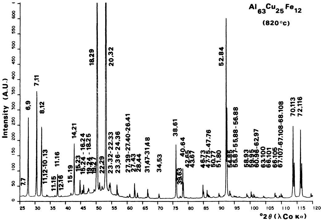
Fig. 6. — X-ray powder diffraction pattern of the single-phase \text{Al}_{63}\text{Cu}_{25}\text{Fe}_{12} icosahedral alloy. The alloy has been quenched by planar flow casting, then the flakes have been annealed for 2 h at 1 093 K.
