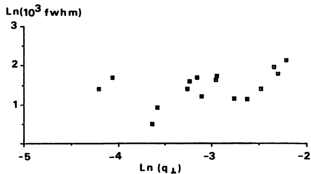
Fig. 4. — Icosahedral glass model : plot of the peak width (fwhm) as a function of the perpendicular component of the 6D wave vector.
