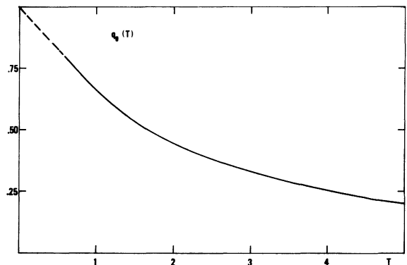
Fig. 2. — The overlap q_0 between relevant tours at temperature T (see (4.5)). The curve for T > 0.6 is obtained from the high temperature expansion, and then extrapolated linearly.
