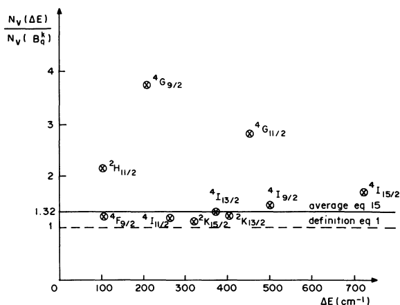
Fig. 1. — Ratio of N_v parameters obtained from \Delta E (Eq. (15)) and from B_q^k (Eq. (1)) versus the maximum splitting of J -terms ( \Delta E ) of \text{Nd}^{3+} in \text{LaF}_3 . Splittings and B_q^k are taken from [12]. The horizontal line shows the proportionality of \Delta E with N_v for several J -terms according to equation (15).
