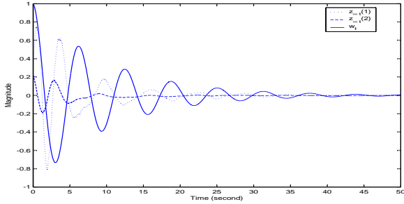
Fig. 2. Evolution of the controlled outputs z_{\infty t} : single sample path simulation
