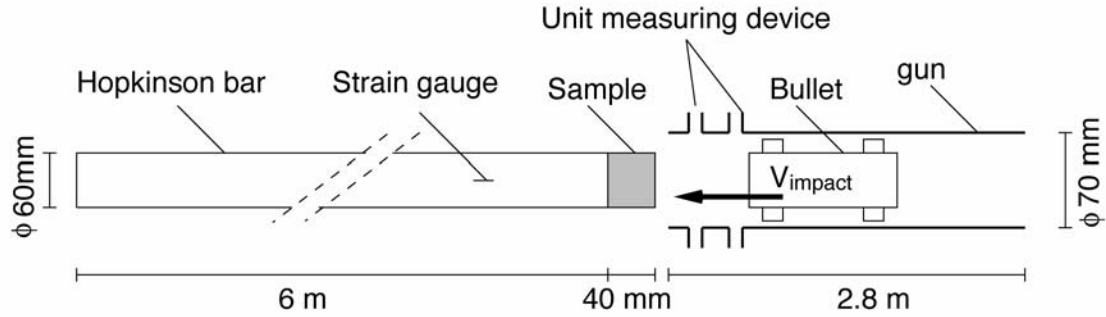
a) Configuration 1: direct impact Hopkinson bar test
