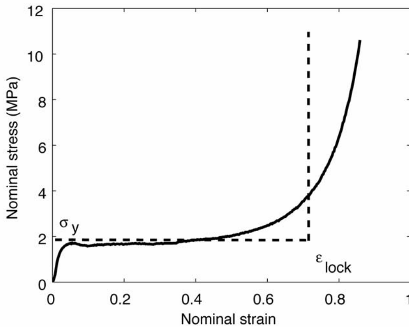
Figure 3. Simplified Rigid Perfectly Plastic Locking model
