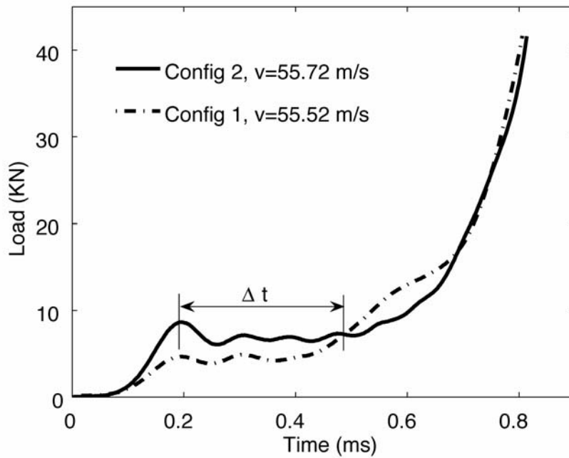
Figure 8. Force profile ahead of (config. 1) and behind (config. 2) the shock front for Alporas foam
