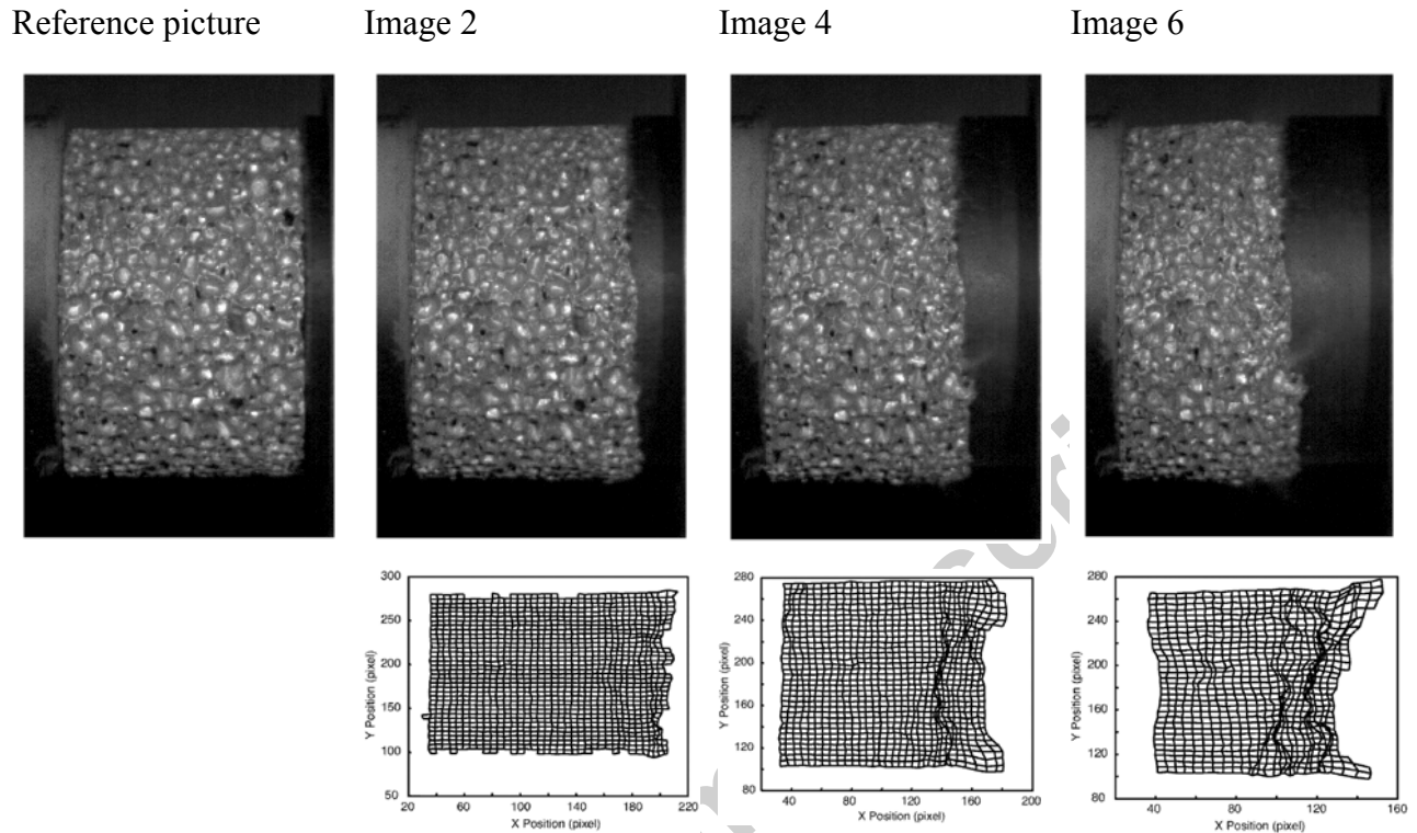
Figure 15. Raw images taken by the camera. Impact velocity of 47 m / s, acquisition rate: 20,000 fps. Corresponding deformed mesh calculated with a Q4P1 correlation algorithm.
