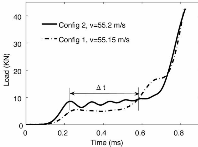
Figure 9. Force profile ahead of (config. 1) and behind (config. 2) the shock front for nickel hollow spheres
