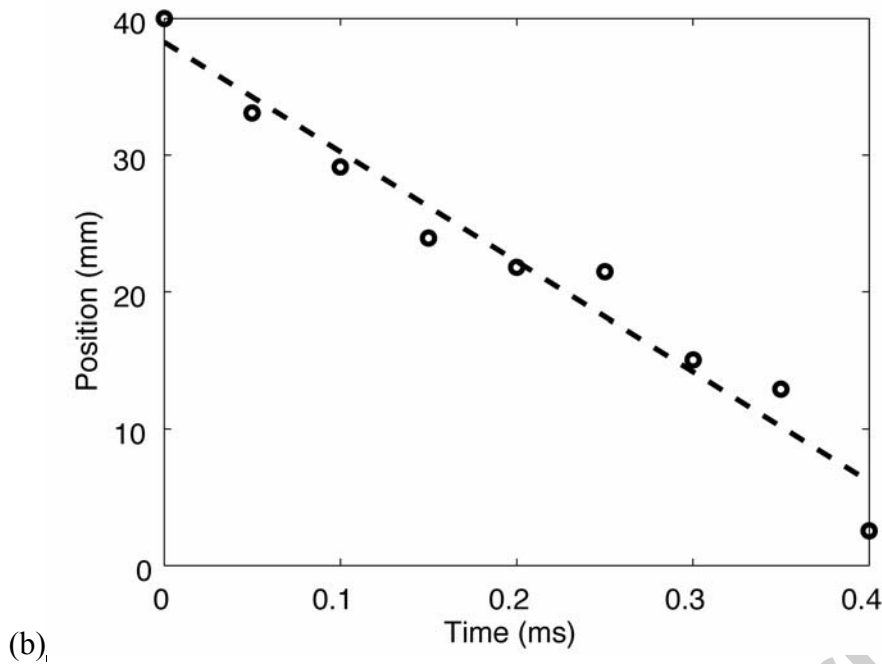
Figure 17. Position of the shock front with time for two impact velocities: 47 m / s (a) and 56 m / s (b)
