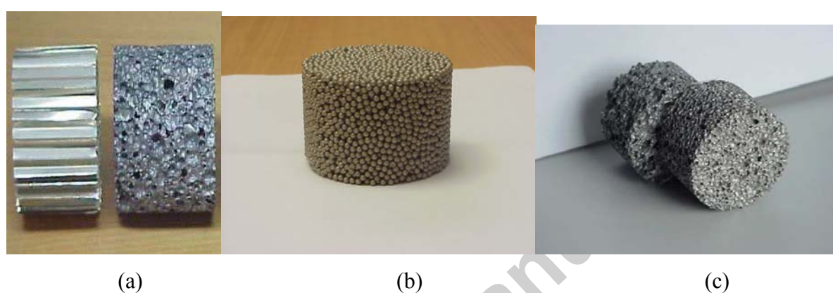
Figure 6. Honeycomb and Cymat foam (a), Hollow spheres (b), Alporas foam (c) specimens (diameter: 60 mm, length: 40 mm)
