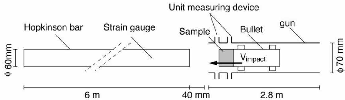
b) Configuration 2: Hopkinson bar-Taylor test
