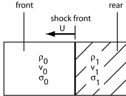
Figure 2. Shock front within a foam-like specimen
