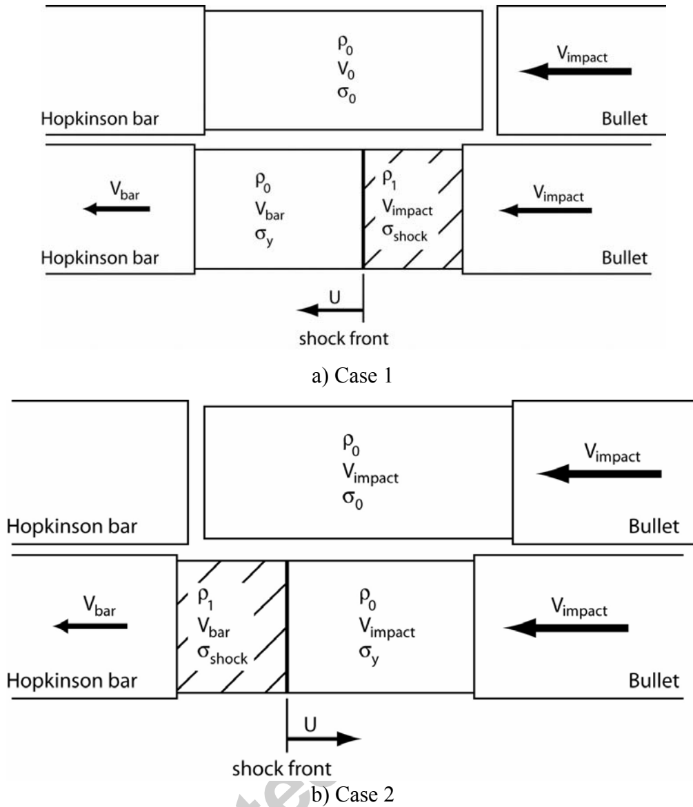
Figure 5. Depiction of the shock front in the two different testing configurations
