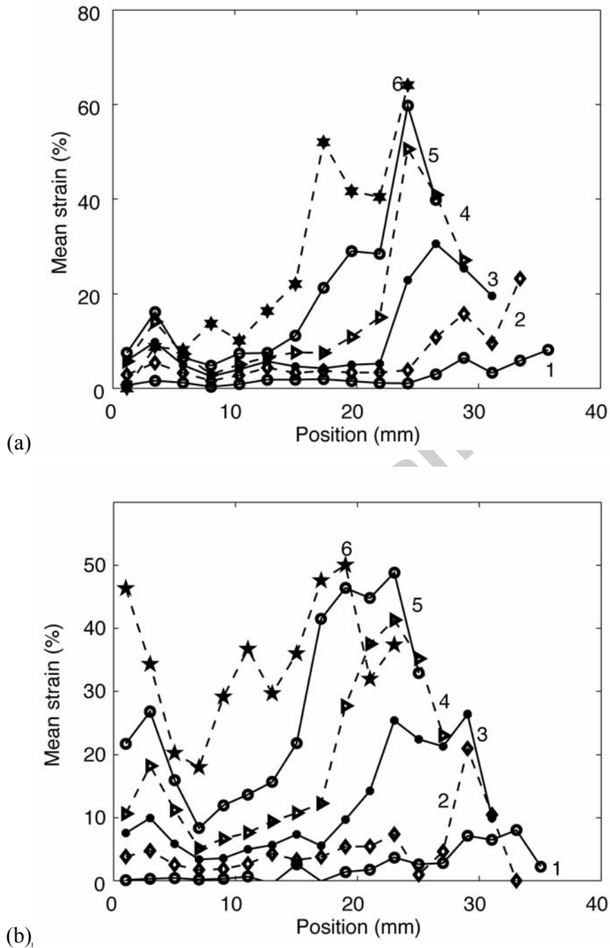
Figure 16. Change of the mean longitudinal strain in the specimen impacted at a) 47 m / s b) 56 m / s (solid line: even numbers of images, dashed line: odd numbers of images)
