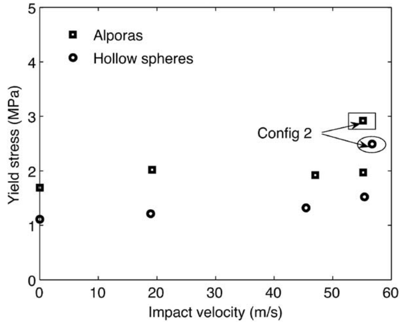
Figure 10. Summary of testing results for Alporas foam and nickel hollow spheres
