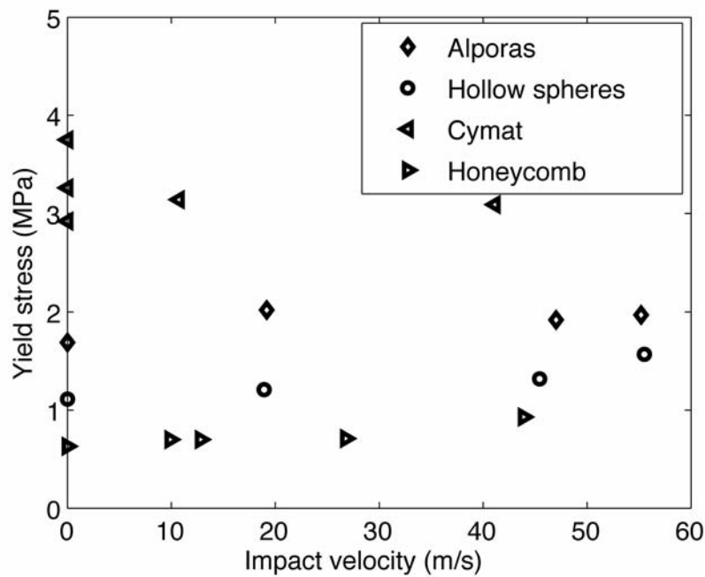
Figure 13. Rate sensitivity of the tested cellular materials
