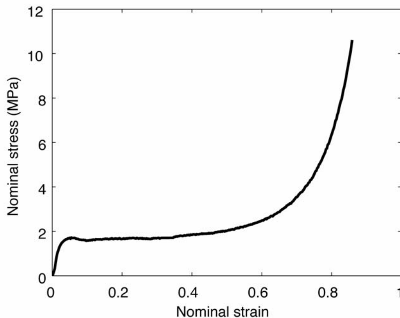
Figure 1. Typical stress-strain relation of a foam-like material (Alporas, 245 \text{ kg/m}^3 )
