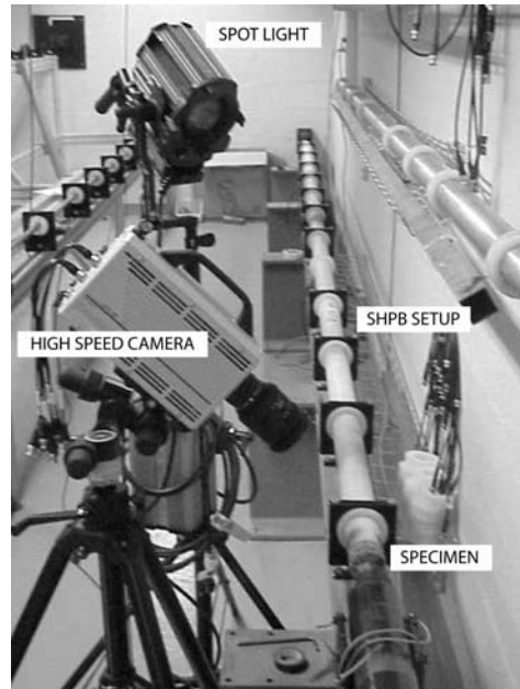
Figure 14. Experimental setup for image capture
