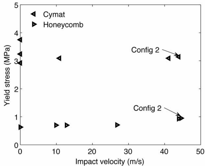
Figure 11. Summary of the testing results for honeycomb and Cymat foam
