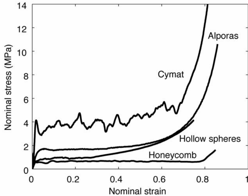
Figure 7. Typical quasi-static stress / strain response of the tested materials
