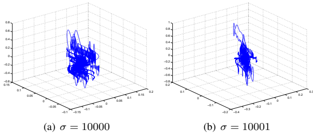
Fig. 10. Attractors for near values of \sigma
