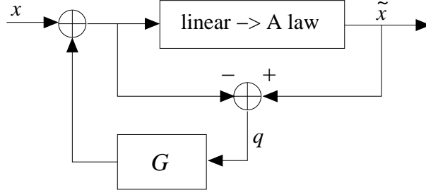
Fig. 17. Noise shaping using a feedback loop.
