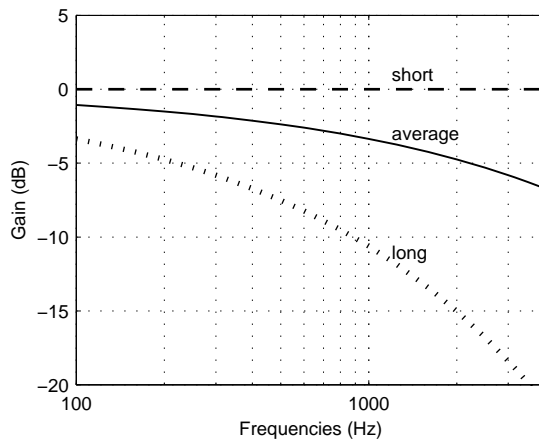
Fig. 5. Frequency responses of different customer lines.
