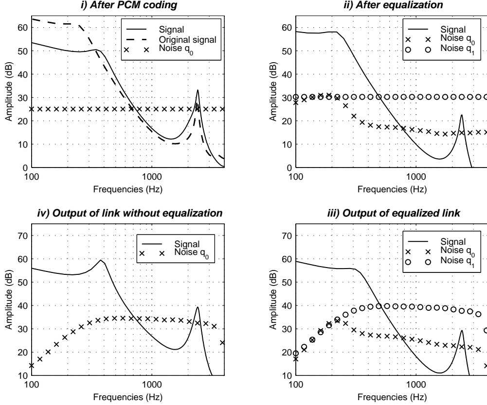
Fig. 16. Spectral envelope of [Y] and corresponding quantization noises in different parts of the link.
