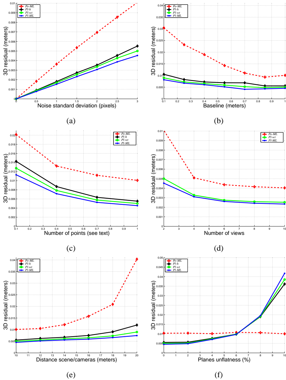
Figure 1: Comparison of the 3D residuals for different approaches versus different scene parameters. Note that method PI-h is not visible on (d) since it works with two views only.
