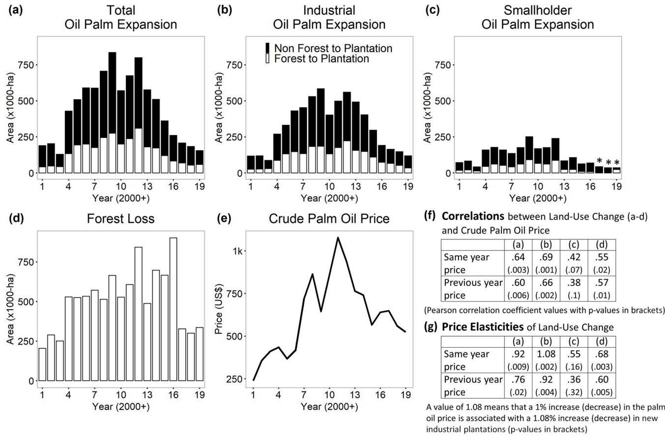
Fig 2. Time-series of Indonesia's land-cover/use change from 2001 to 2019. Expansion of oil palm plantations by year (a), split between industrial and smallholder (b,c). Forest loss (d). Mean annual Crude Palm Oil price (e). Correlations/elasticities with the previously shown land-cover change estimates (f,g). Price calculated from monthly prices in USD using IMF data [29]. In insets (a,b,c) white bars represent the areas of forest cleared and converted to plantations in the same year. This rapid conversion constitutes 29% of all forest loss detected during 2001–2019. The black bars represent areas of non-forest converted to oil palm. Ninety six percent (5.39 Mha) of those non-forest areas were non-forest in 2000, 4% (0.24 Mha) were forest cleared after 2000 and converted to plantations more slowly (after 2 to 18 years). These non-forest areas include conversion of young regrowth, mixed gardens, agroforests, and rubber plantations. Asteriks (*) indicate that the area of smallholder expansion in 2017, 2018, 2019 is likely underestimated. We note that the 2016 peak in forest loss (d) includes losses of late 2015, when fire burned large areas of forest in Kalimantan. Much of these losses were recorded only the following year by the Tree Loss dataset used to calculate forest loss because of cloud cover.
