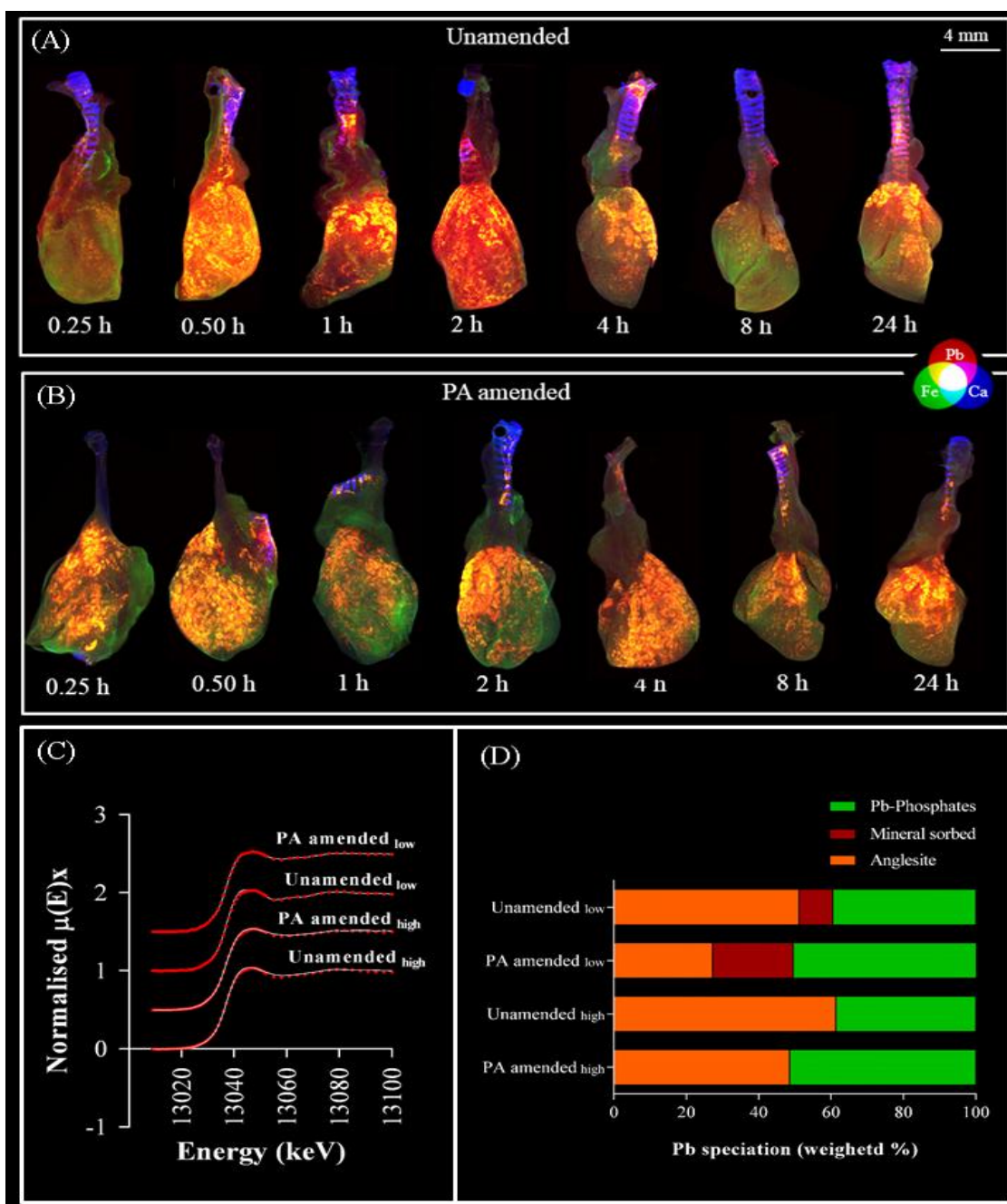
Figure 3: (A) and (B) 2D Elemental map (Pb = red, Fe = green and Ca = blue) using X-ray Fluorescence Microscopy (XFM) in mice lungs (including partial trachea) exposed to unamended and phosphoric acid (PA) amended dust via instillation over 24 h. (C) Pb speciation in regions of interest in the 24 h mouse lungs using X-ray Absorption Near Edge Structures (XANES). Linear combination fitting (LCF) is indicated using red dots and original spectra as white lines. (D) Final Pb speciation (weighted %) results obtained using XANES.
