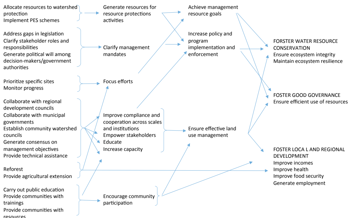
Figure 10. Means-ends objectives diagram summarizing stakeholder preferences for successful EBA in the Guacerique watershed
