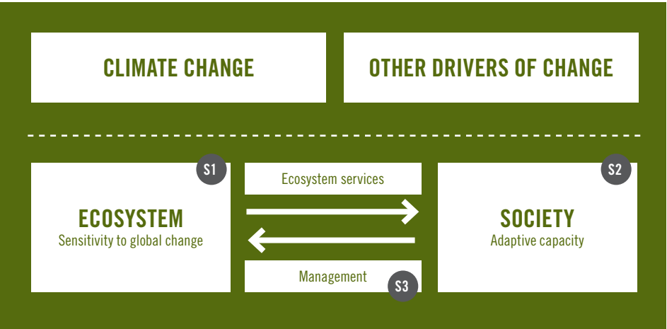
Figure 6. Framework for the vulnerability assessment
