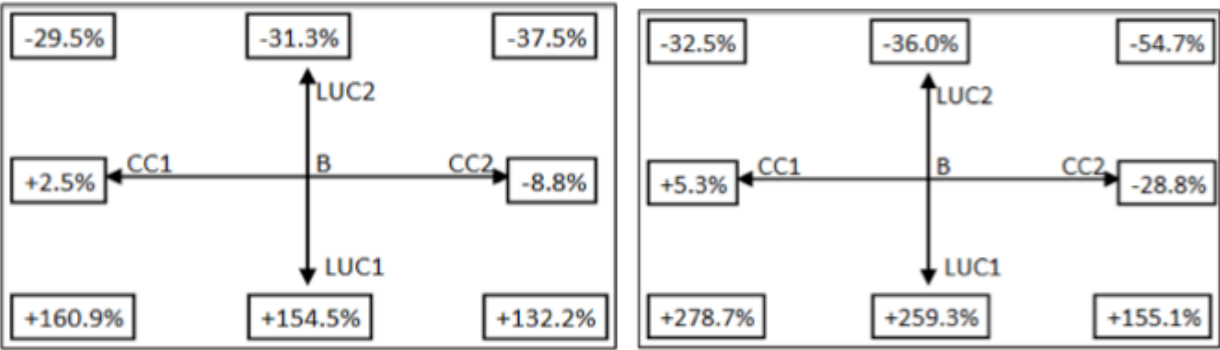
Figure 7. Change in soil erosion compared with the baseline (B) for two contrasting climate scenarios (CC1 – PCM.B2A and CC2 – HAD3.A1FI) and two contrasting land use change scenarios (LUC1 – Scenario A and LUC2 – Scenario D) in 2030 (left) and 2080 (right)
