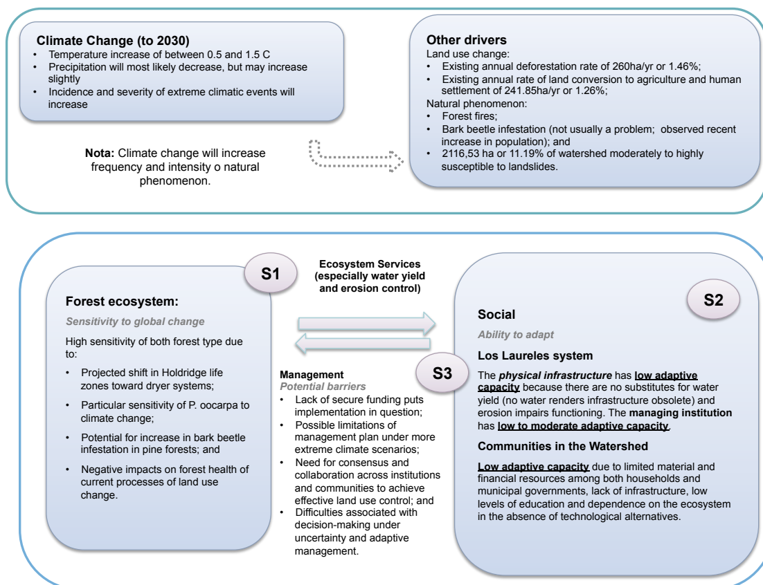
Figure 8. Vulnerability analysis for the Guacerique watershed
