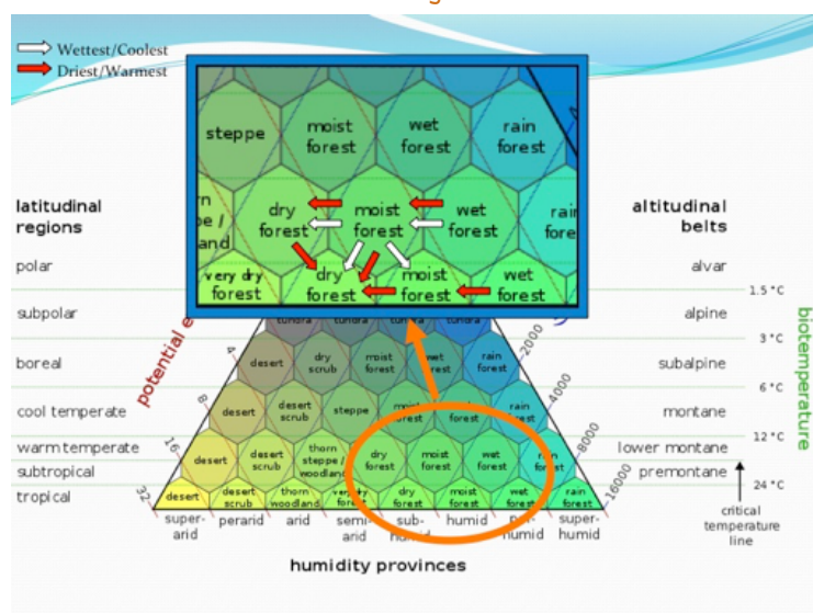
Figure 9. Results of modeling of changes to life zones in the province of Francisco Morazán under climate change
