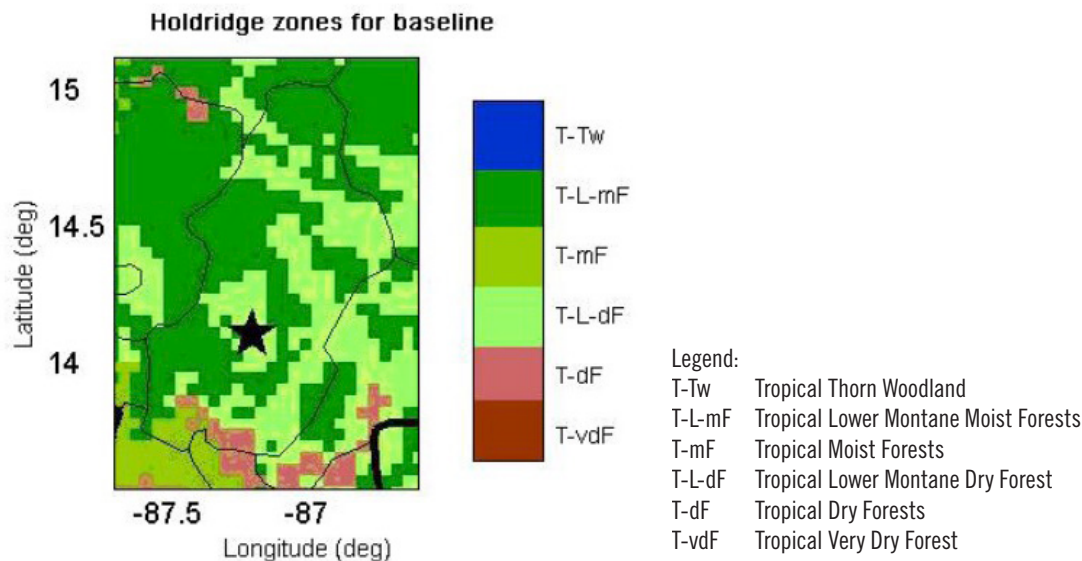
Figure 2. Current Holdridge life zones in the province of Francisco Morazán, Honduras
