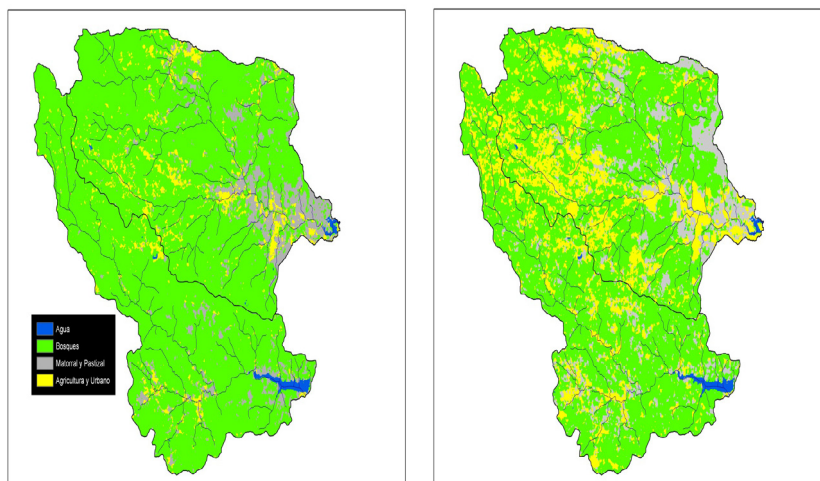
Figure 3. Land use change in the Guacerique and Grande watersheds, 1993–2008
