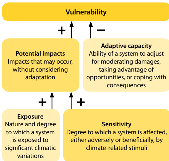
Figure 4. Vulnerability as a function of exposure, sensitivity and adaptive capacity
