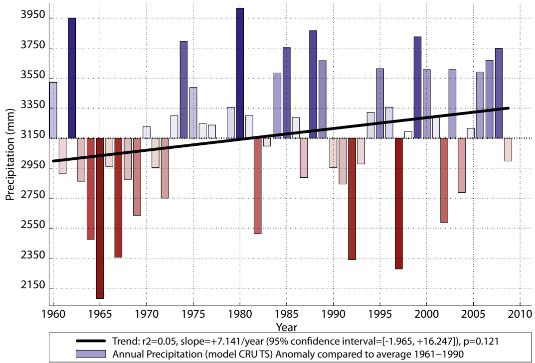
Figure 9. Variability in annual precipitation in Malinau, 1960–2010
