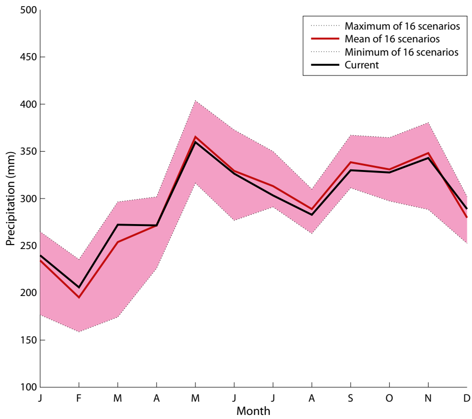
Figure 12. Predicted monthly precipitation in Malinau for 2080
