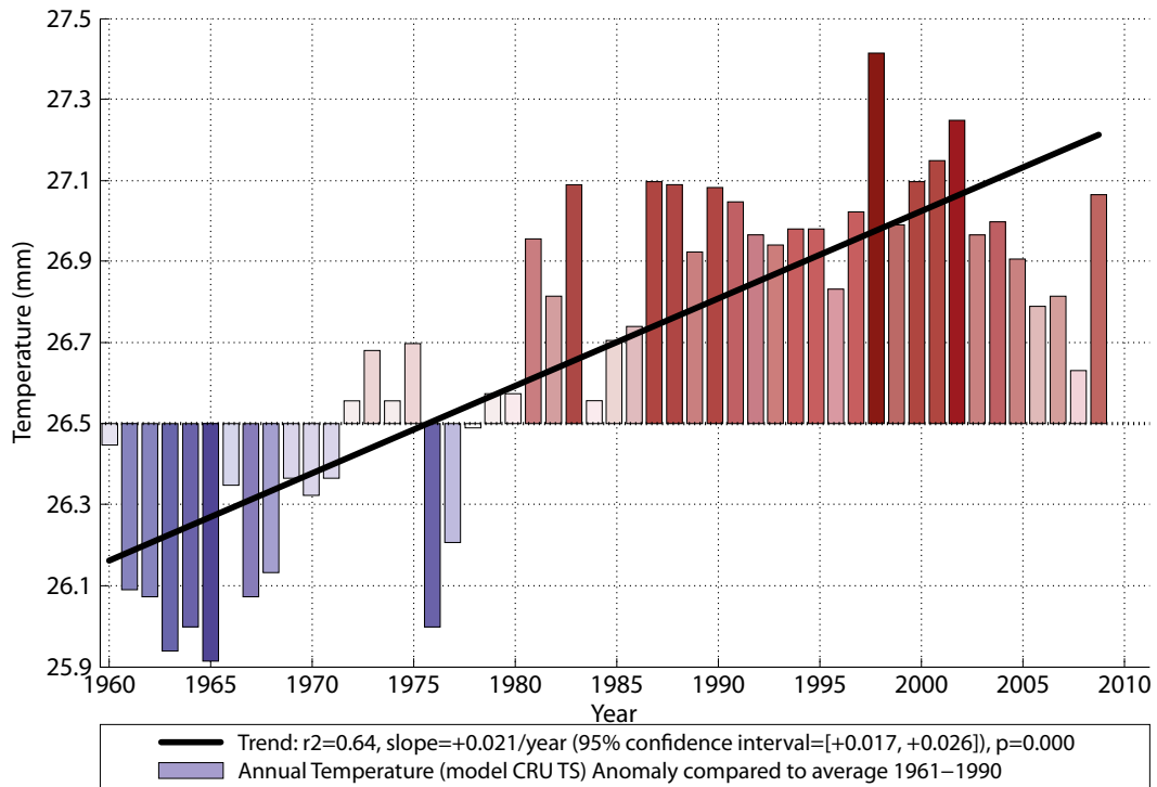
Figure 10. Variability in annual temperature in Malinau, 1960–2010
