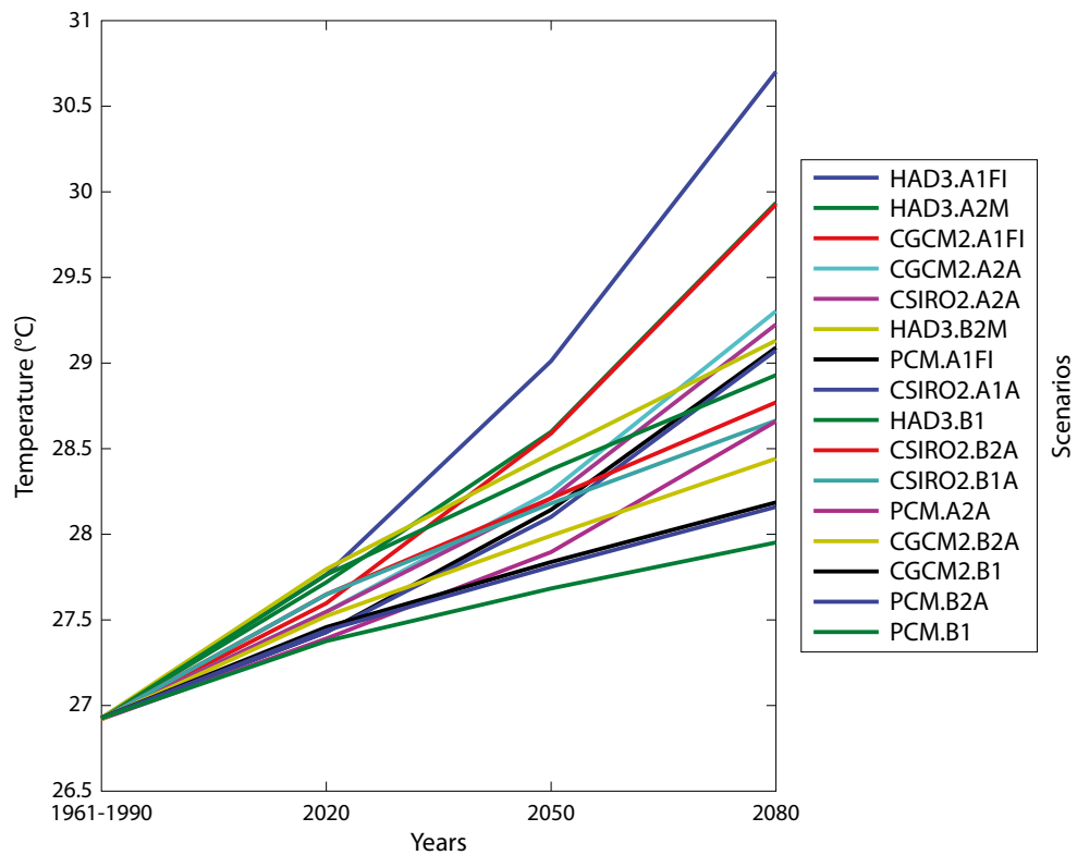
Figure 13. Mean temperatures in Malinau in 2020, 2050 and 2080, according to 16 climate scenarios
