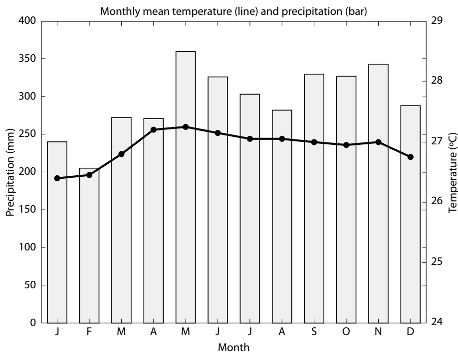
Figure 8. Average climate in Malinau
