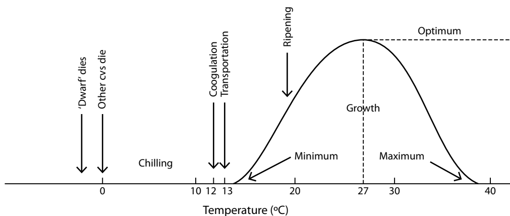
Figure 14. Relationships between temperature and banana growth
