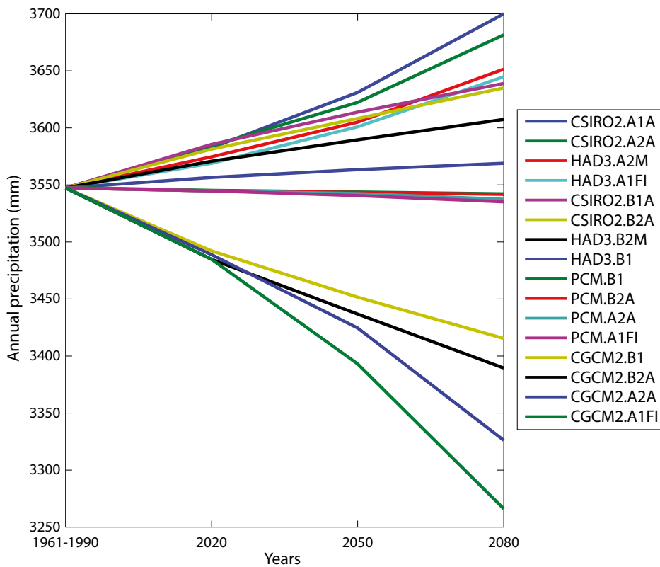
Figure 11. Annual precipitation in Malinau in 2020, 2050 and 2080, according to 16 climate scenarios
