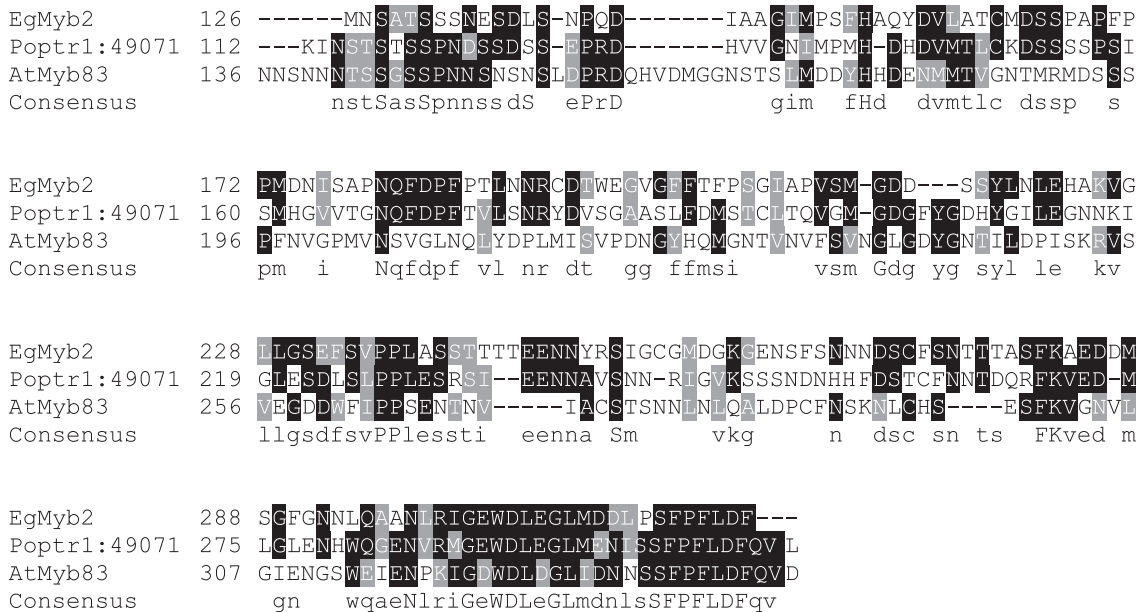
Figure 2. Sequence analysis of the EgMYB2 protein.
