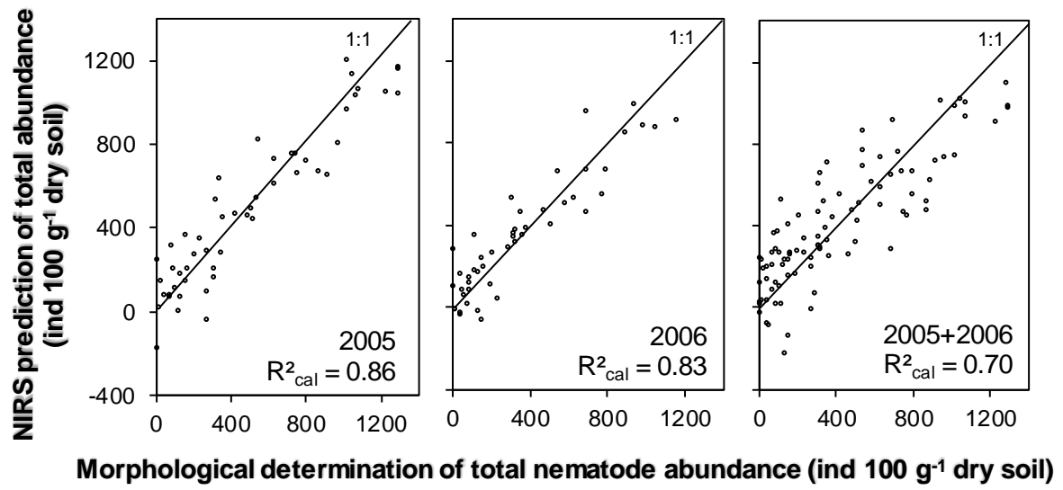
Figure 1. Comparison between morphological determination and NIRS prediction of total nematode abundance for the yearly sets and for the total set.
