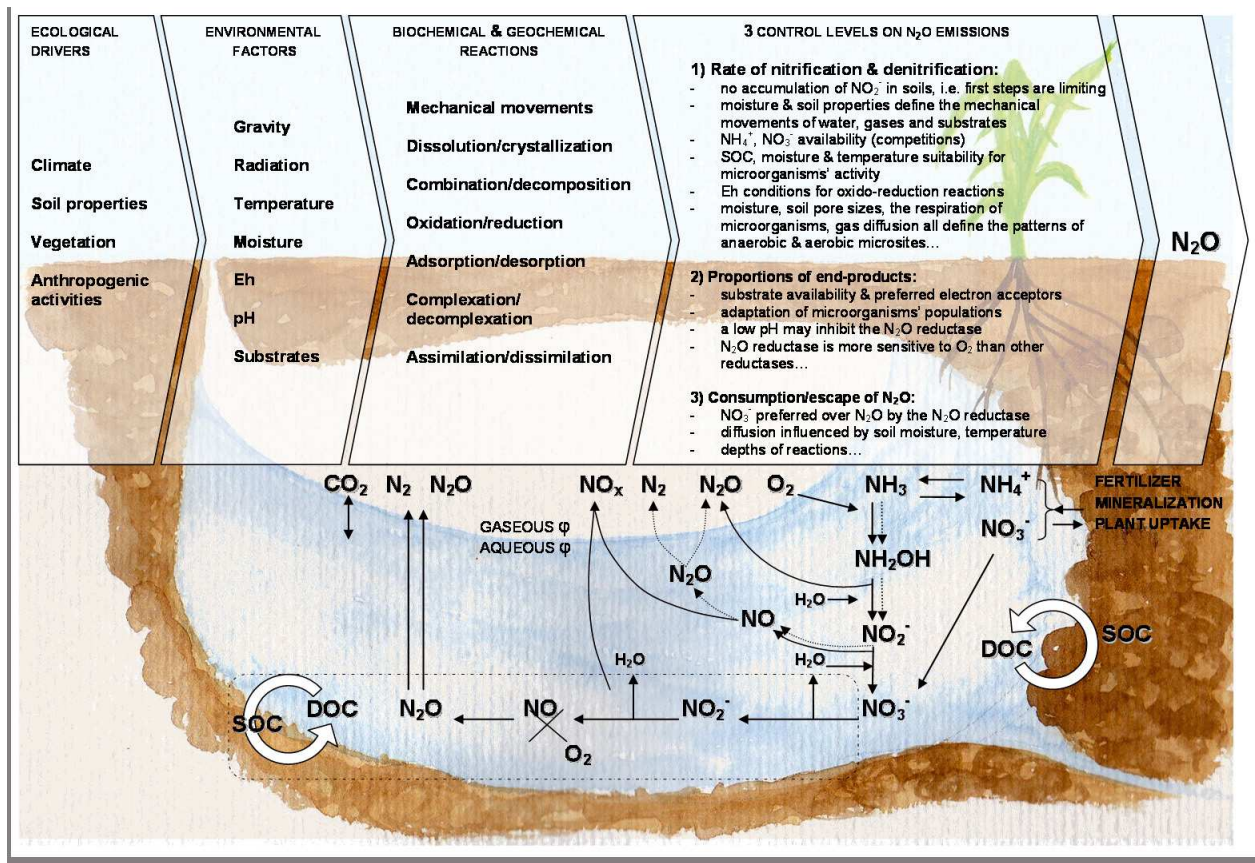
Figure 15. Scheme of the determinism of N_2O emissions by soils adapted from Li (2007); Wrage et al. (2005); Farquharson and Baldock (2008). Soil particles, gaseous and aqueous phases ( \phi ) are artificially “well distinguished”. The two extremities of the symbolised pore represent the pore continuum throughout the soil matrix. Reactions take place at the interface of soil particles and aqueous phase where microorganisms and substrates are. Denitrification takes place in the “anaerobic dashed-line rectangle”. Dashed arrows lead to N_2O emissions by nitrifier denitrification occurring in low O_2 conditions, which implies that some NH_3 oxidisers process the whole reaction chain (Wrage et al., 2001).
