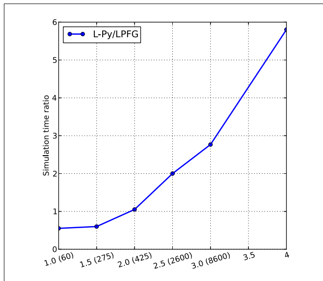
FIGURE 14 | Computation time comparison with between L-Py and lpfg for MAppleT. The horizontal axis represents age of the simulated tree with estimated number of elements of the tree.
