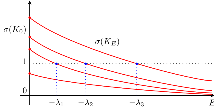
FIGURE 5.3 – Le principe de Birman-Schwinger.
