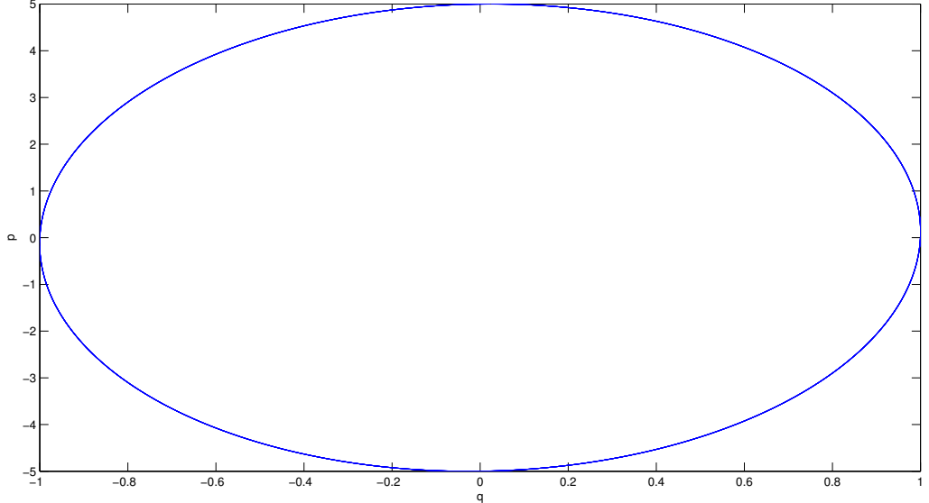
Figure 6: Symplectic Euler scheme, T = 10 , h = 0.01 . Upper figure: solution in the (q, p) plane. Lower figure: Evolution of the energy.
