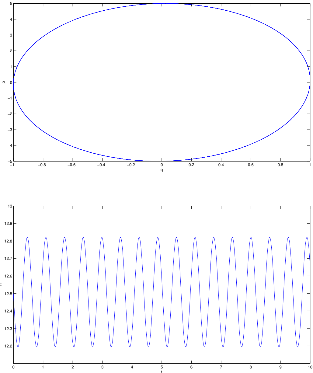
Figure 6: Symplectic Euler scheme, T = 10 , h = 0.01 . Upper figure: solution in the (q, p) plane. Lower figure: Evolution of the energy.
