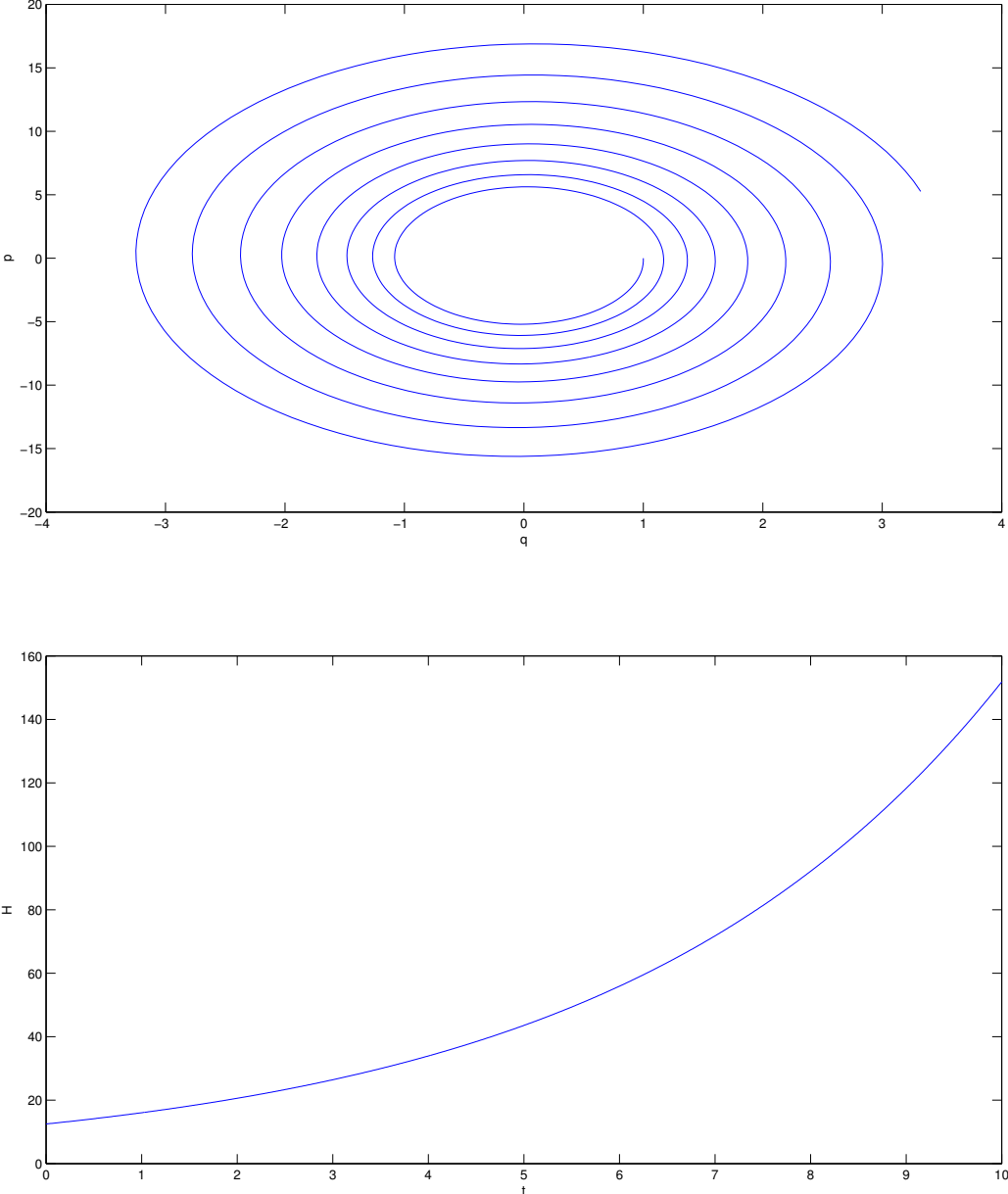
Figure 2: Explicit Euler scheme, T = 10 and h = 0.01 . Upper figure: solution in the (q, p) plane. Lower figure: Evolution of the energy.
