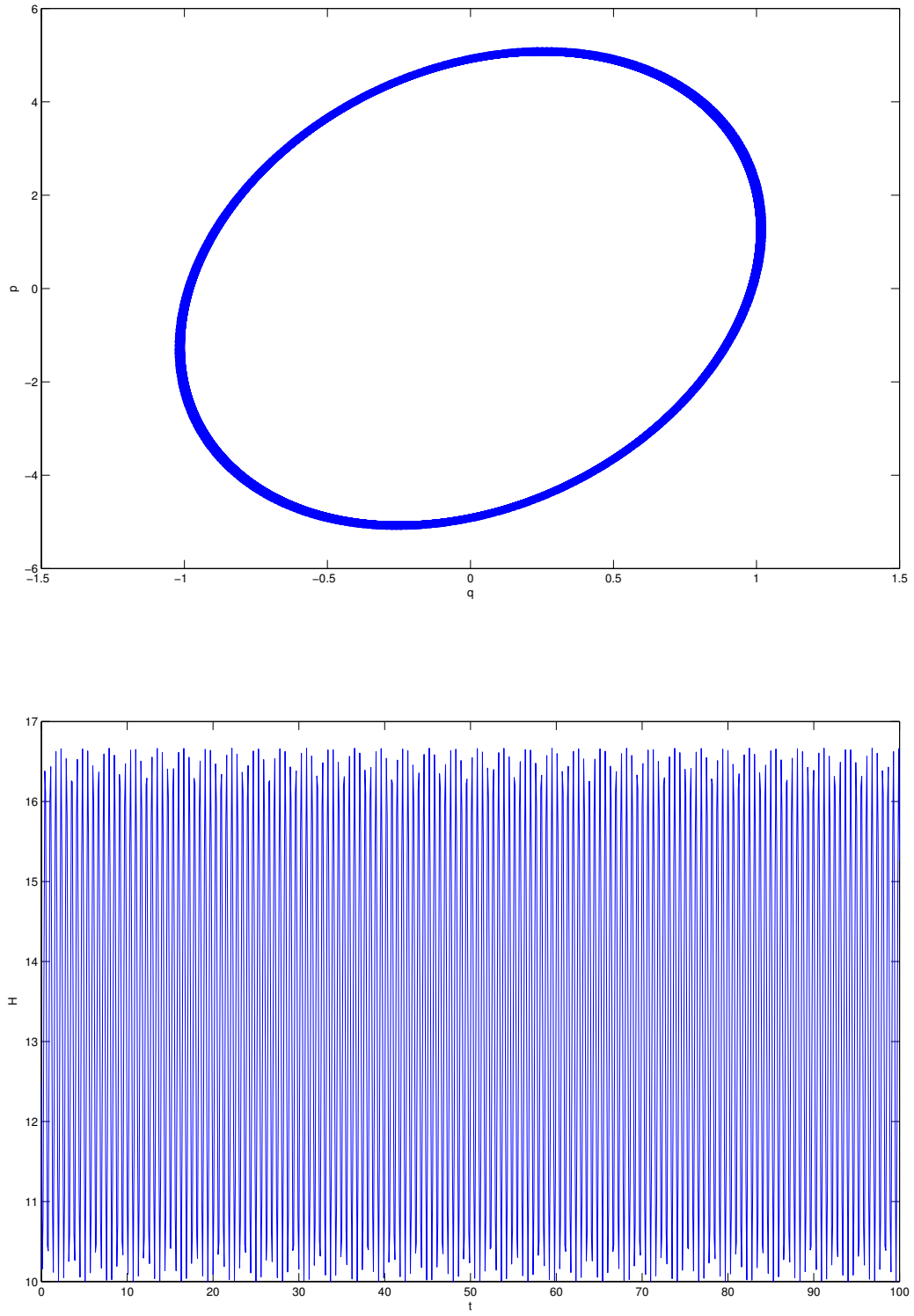
Figure 7: Symplectic Euler scheme, T = 100 , h = 0.1 . Upper figure: solution in the (q, p) plane. Lower figure: Evolution of the energy.
