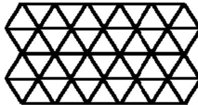
Hexagonal graph
