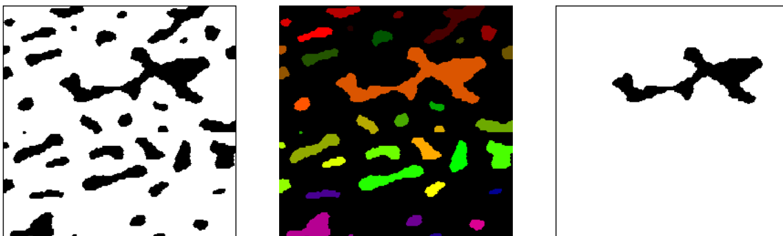
Thresholding the labelled image (middle) at 12 extracts the twelfth particle (right) of the initial binary image (left).
