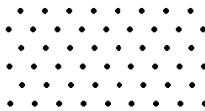
Hexagonal grid
