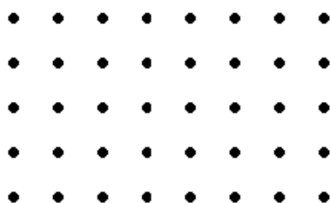
Square grid
