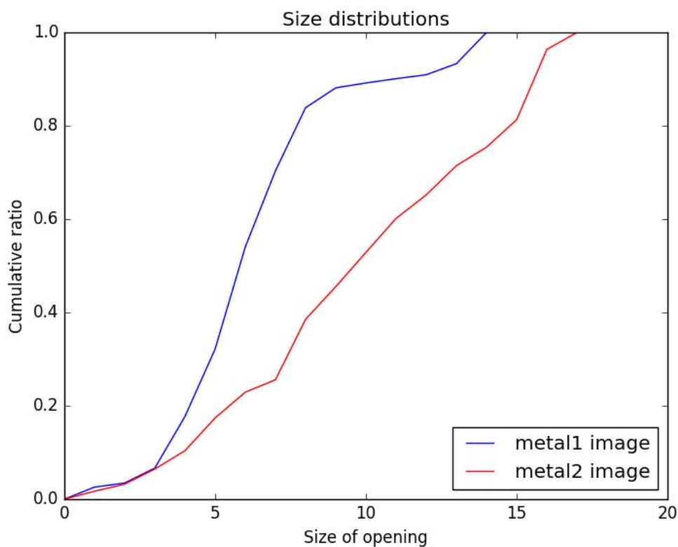
Size distributions (hexagonal openings) of the metal1 and metal2 images.
