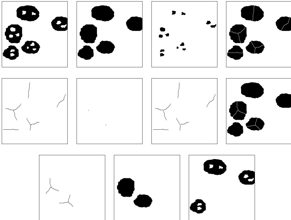
From left to right and from top to bottom: initial image (particles with at least two holes), particles without holes, holes, geodesic SKIZ of the holes, boundaries of the SKIZ, multiple points, simple arcs of the SKIZ, second geodesic SKIZ of the simple arcs, boundaries of the second SKIZ, reconstructed particles (particles with more than two holes), final result (particles with two holes).
