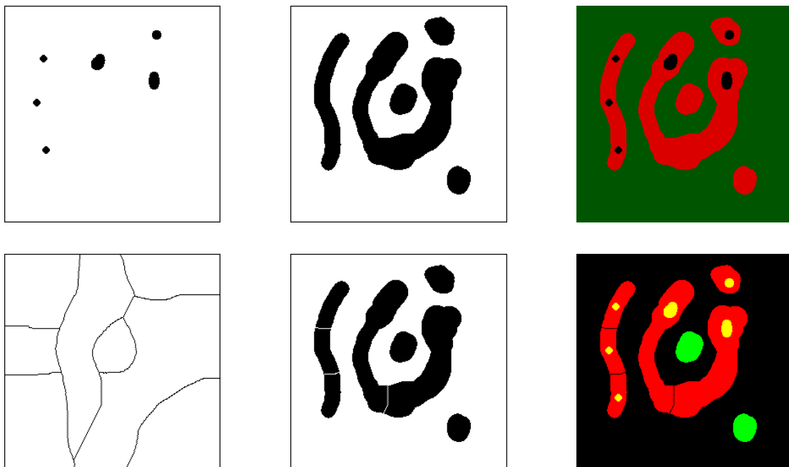
Upper left: initial set (holes of the test_geodSKIZ image). Upper middle: geodesic space (test_geodSKIZ image without holes). Upper right: function used for the watershed, black points take value 0, red ones take value 1 and green ones take value 2. Lower left: watershed transform of the previous function. Lower middle: influence zones together with the connected components of the geodesic space at an infinite geodesic distance from the initial set. Lower right: in yellow, initial set, in red influence zones in the geodesic space, in green connected components which do not belong to any influence zone.
