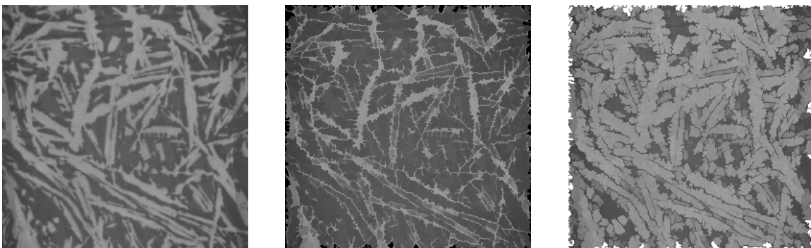
ferrite1 image (left), its full thinning with the hexagonalL structuring element (middle) and its full thickening with the same structuring element (right).
