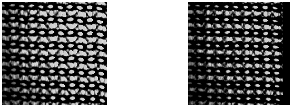
The erosion of the left greyscale image by a doublet of points at distance 25 with the edge set to EMPTY produces a black strip, as shown in right image.
