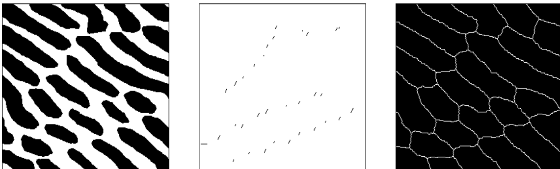
Original opened image (left), extreme points (middle) and influence zones of the lamellae (right).
