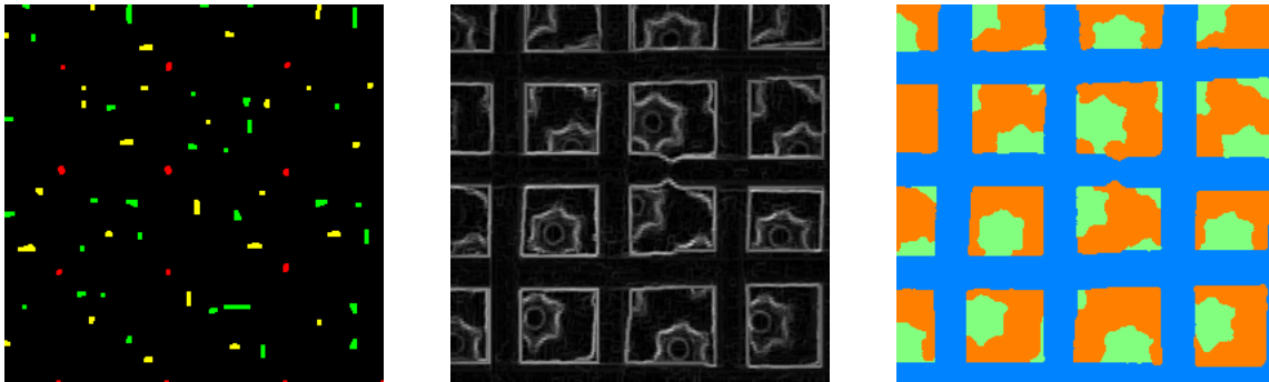
Left: markers of the background (in green), of the hexagonal structures (in yellow) and of the raster (in red). Middle: supremum of the gradient images of the initial filtered image and of the raster image. Right: watershed segmentation.
