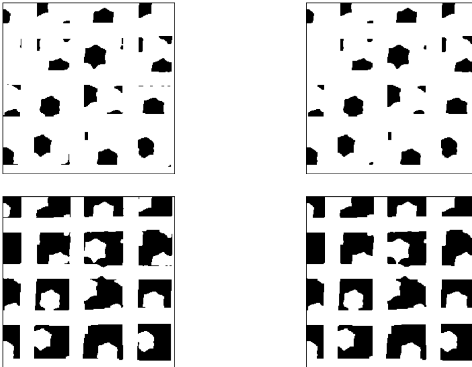
Hexagonal structures extracted by thresholding (upper left), their opening (upper right), background (lower left) and its opening (lower right).
