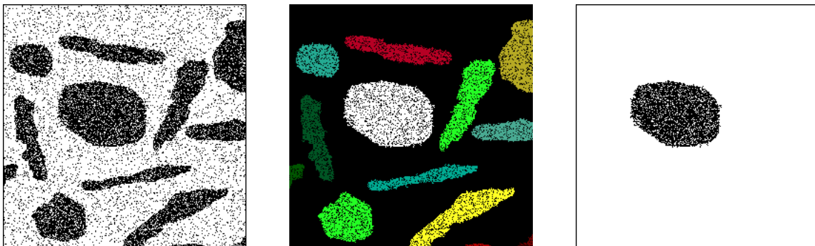
Initial noise image (left), labelling of the connected components by their number of holes + 1 (middle), Extraction by thresholding of the connected component with a label equal to 485 (right). Its connectivity number is equal to -483. This connected component contains 484 holes.
