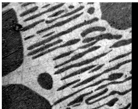
Display of the image alliage. The image is padded with 0 (right stripe) to adjust its size (480x400) with the MAMBA image size (512x400).
