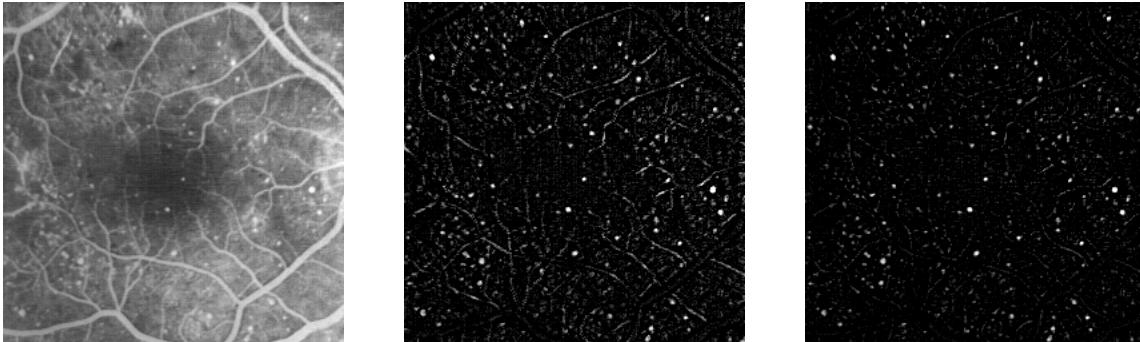
Retina2 image (left), top-hat with a sup of linear openings (middle) and top-hat when a geodesic reconstruction is performed before the subtraction (right). Some parts of vessels still remaining in the middle image have totally disappeared in the right one.
