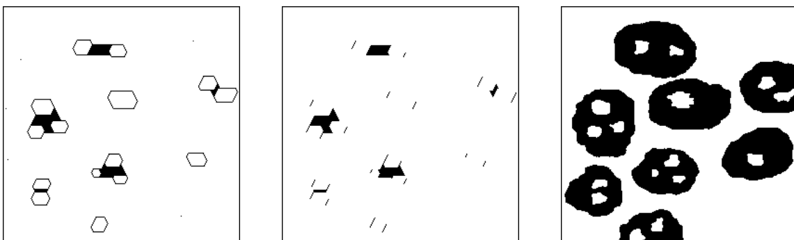
Thinning with D (left), linear erosion in direction 1 - but any direction can be used (middle), reconstruction of the particles with hole(s) with the previous erosion as marker image (right).
