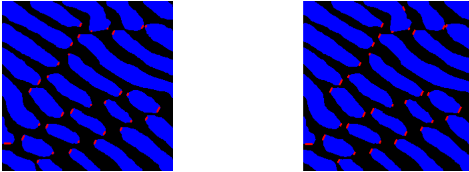
Detection of the extremities of the opened eutectic image (right) compared to the detection by extracting the maxima of the opened geodesic distance function (left).
