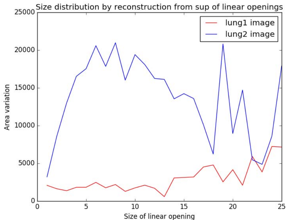
Size distribution curves with a geodesic reconstruction from a sup of linear openings for the lung1 and lung2 images.
