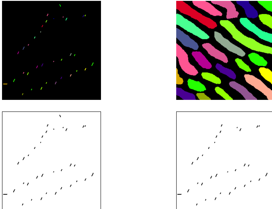
From top to bottom and from left to right: valued extremities of the eutectic image, labelling of the lamellae by the greatest geodesic distance of the points from the geodesic center (corresponds to half the length of the particle), extremities and extreme points.
