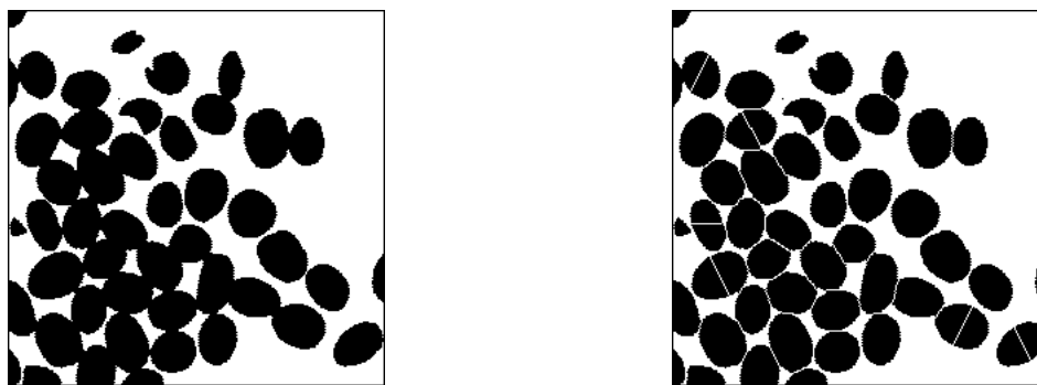
Original coffee image (left) and result of the segmentation by the segmentParticles operator (right). Some coffee grains are over-segmented. Note also that a grain on the upper left side is badly segmented.
