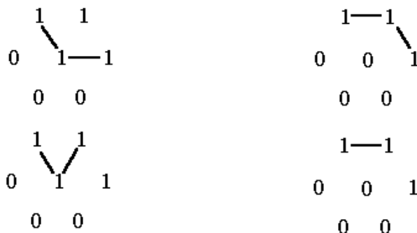
Initial paths before thinning (left) and equivalent paths after thinning (right). The central point has been removed but a path joining the extremities of the initial path can still be defined because the neighborhood points remain after thinning.
