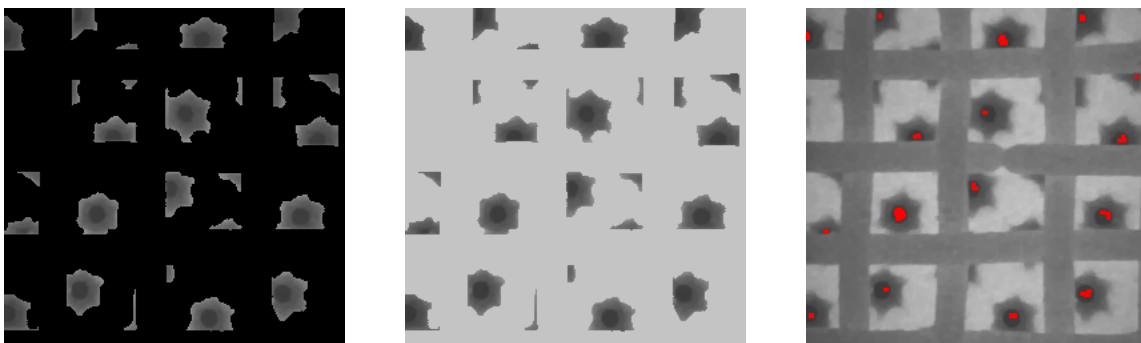
Extracted hexagonal structures (left), filling of the outside (middle), minima with a high dynamics (right, in red).
