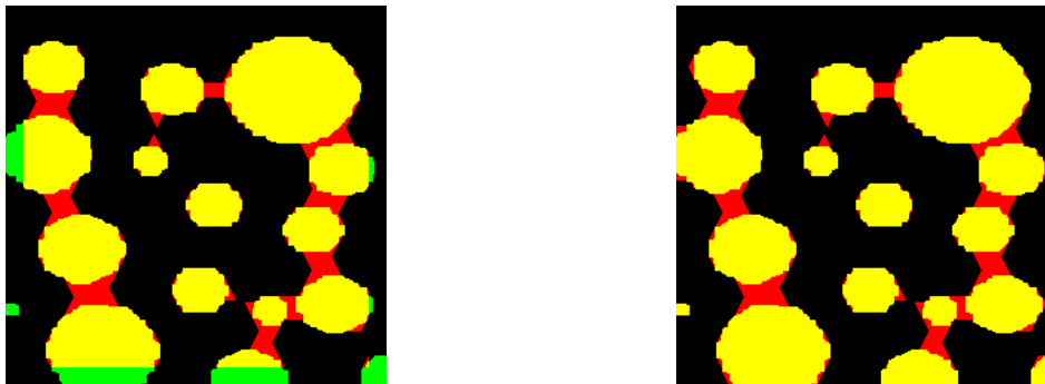
Closing without correction, when the edge is set to EMPTY (left). The operator is not extensive (green part should not exist). Corrected closing (right).
