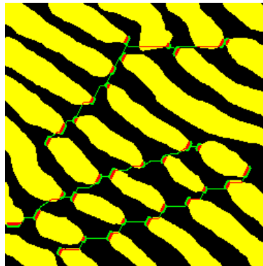
Initial eutectic image (in yellow), extreme points of the lamellae (in red) and dislocation lines (in green).
