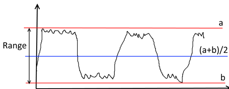
Principle of the automatic thresholding of a two-phased image; the extremal grey values a and b are computed and a threshold can be applied in the middle of the range.
