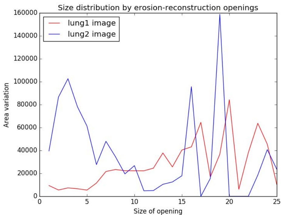
Size distribution curves with erosion-reconstruction openings for the lung1 and lung2 images.
