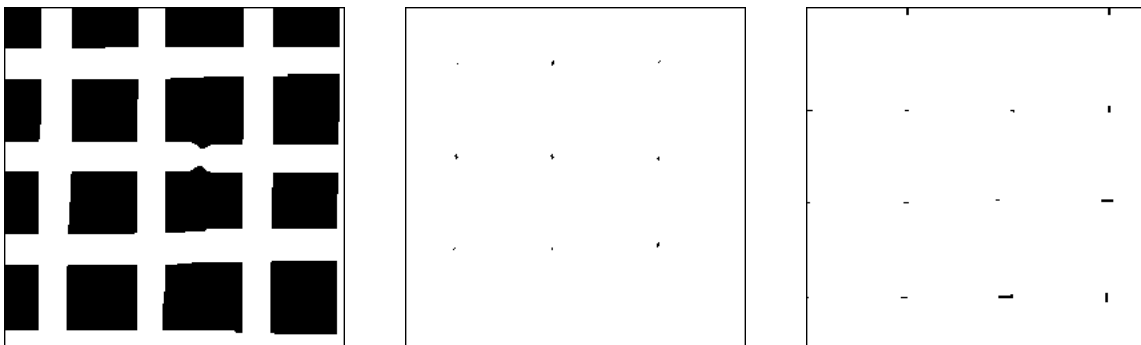
First binary image of the raster obtained by a simple thresholding (left). Markers of the raster (middle) and of the background (right) obtained by ultimate erosions.
