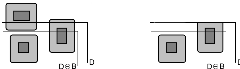
Left image: the set X (dark grey) and its dilation (light grey). Right image: the restriction of X to the field D does not propagate some outside parts of X inside D . The resulting dilation is biased. Only its part inside the erosion of D is correct.
