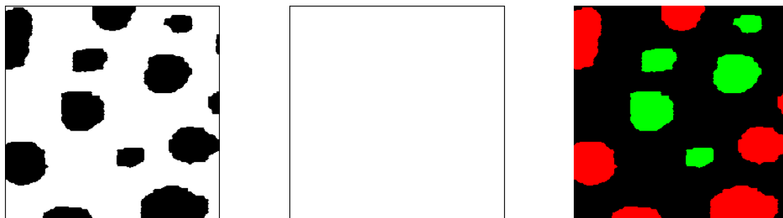
Removal of the objects which touch the edges of the field: initial image (left), marker set (field contour, middle), removed particles in red (right).
