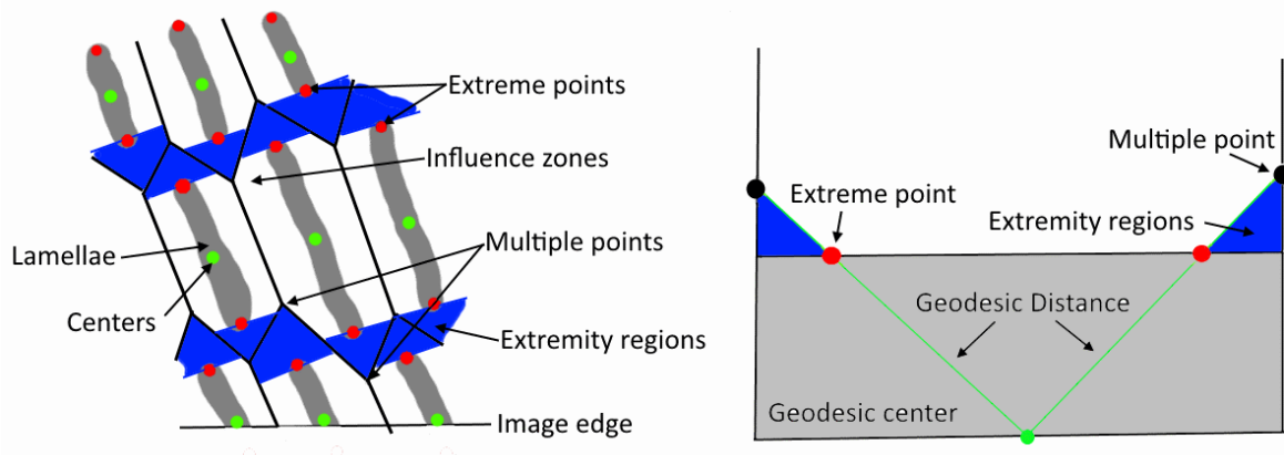
The geodesic centers and the extreme points of the lamellae are extracted. The geodesic distance of the centers inside the influence zones is computed. The influence zones are labelled with the extreme points and are assigned the maximal distance of these points inside each influence zone. The mask of all the points where the geodesic distance is higher than or equal to the labelled image defines the extremity regions.
