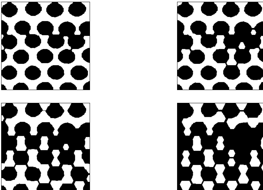
From left to right and from top to bottom: closings of increasing sizes (4, 6, 8 and 10) of the boron fibers.
