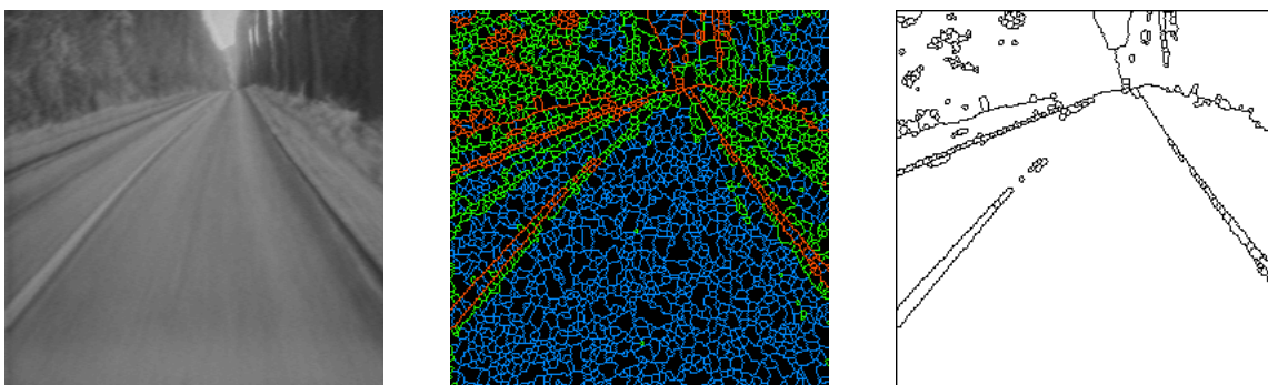
Initial route image (left), result of the enhanced waterfalls segmentation, each level of hierarchy is represented with a different color (middle), extraction of the highest level of hierarchy (right).
