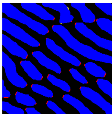
Extreme points of the eutectic image in red. In yellow, extremities which are not farthest points.
