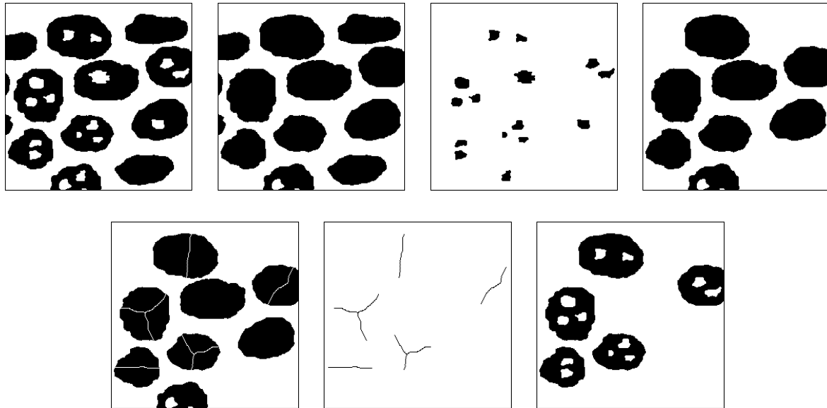
From left to right and from top to bottom: initial image, image with its holes filled, extracted holes, particles with holes (after filling), geodesic SKIZ of the holes in the previous image, boundaries of the SKIZ, geodesic reconstruction of the particles containing at least two holes.
