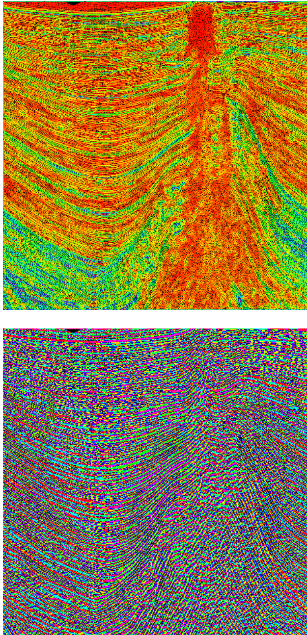
Gradient modulus of the seismic_section image (top), gradient azimuth (bottom) obtained with the vectorialGradient operator.
