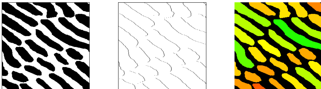
eutectic image (left), its horizontal intercepts (middle) and labelling of each connected component with its vertical diameter (right).
