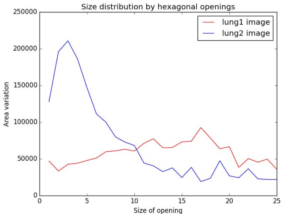
Size distribution curves with hexagonal openings for the lung1 and lung2 images.
