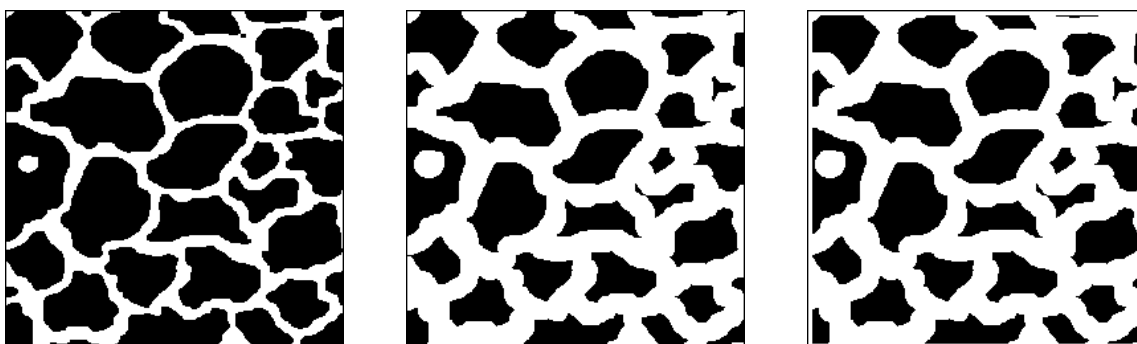
Hexagonal erosion of size 4 of the initial image (left) when the parameter ‘edge’ is set to FILLED (middle) and when set to EMPTY (right).
