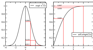
FIGURE 2.2. – Les fonctions \exp(-x^2/2) et \operatorname{erf}(x/\sqrt{2})
