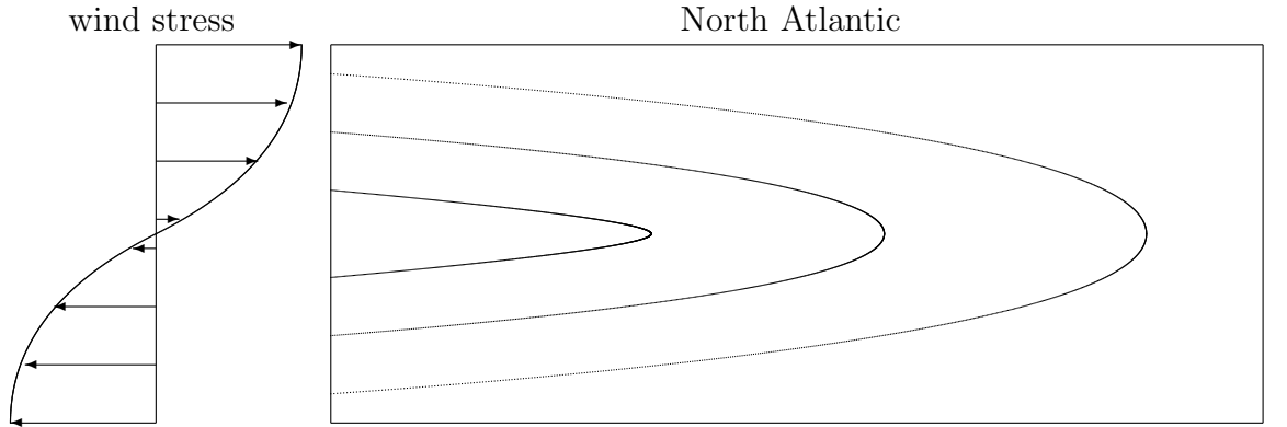
Figure 6.1: Sverdrup Balance: v-component only
