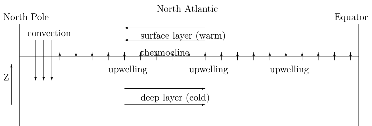
Figure 9.1: Overturning Circulation
