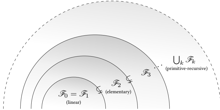
Figure 2.2: The Grzegorzcz hierarchy of primitive-recursive functions.
