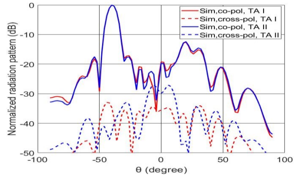
Fig. 8. Simulated normalized radiation patterns in E-plane at 29 GHz for TA-I and TA-II.
