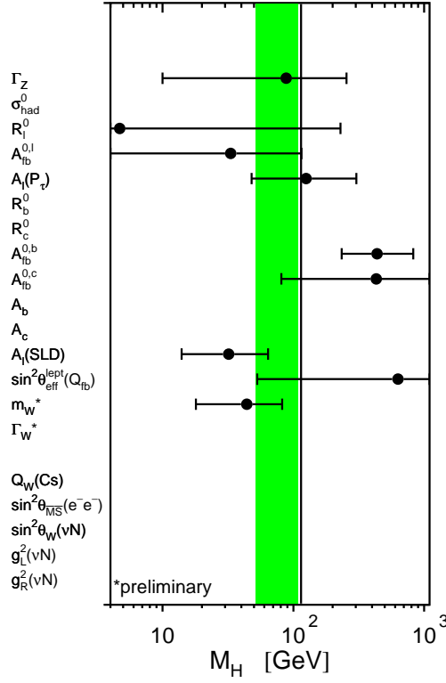
Figure 1: Values of the Higgs mass extracted from different EW observables. The vertical line is the direct LEP lower limit of 114 GeV. The average is shown as a green band [51].
